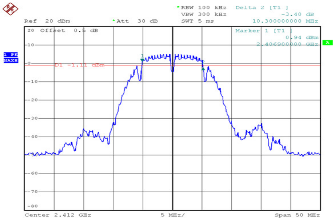
Channel 01 (2412MHz)
