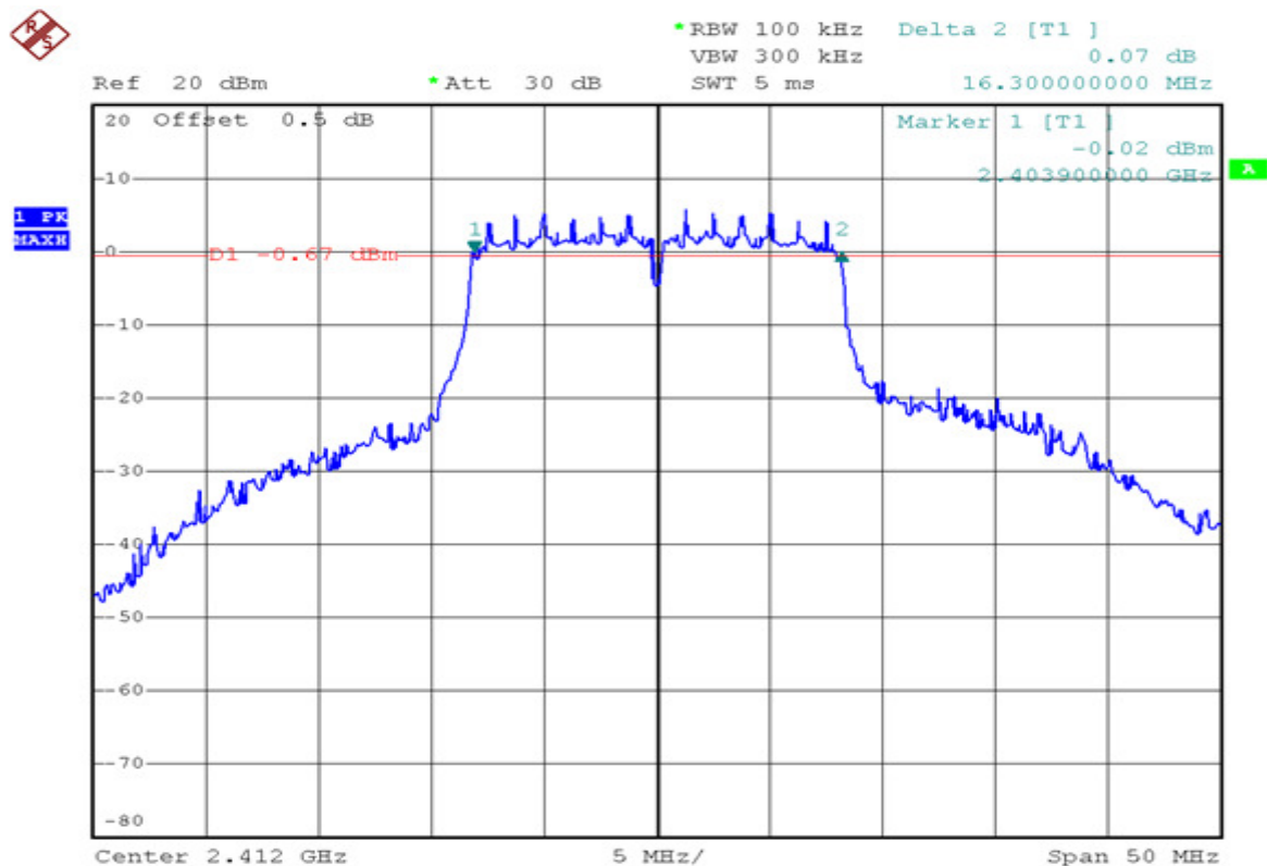
Channel 01 (2412MHz)
