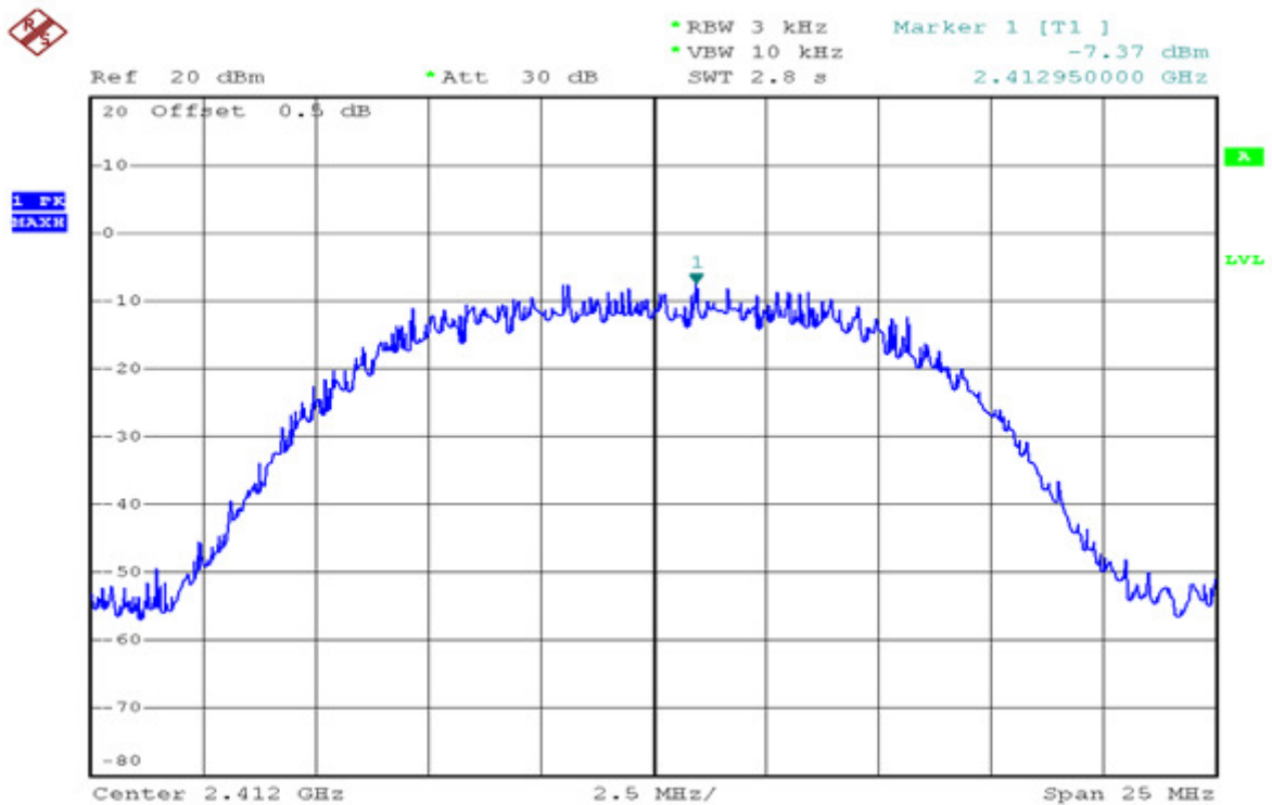
Channel 01 (2412MHz)
