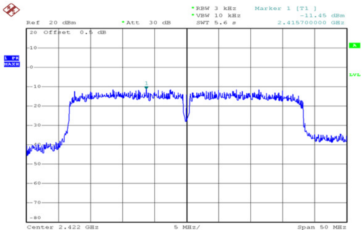
Channel 03 (2422MHz)
