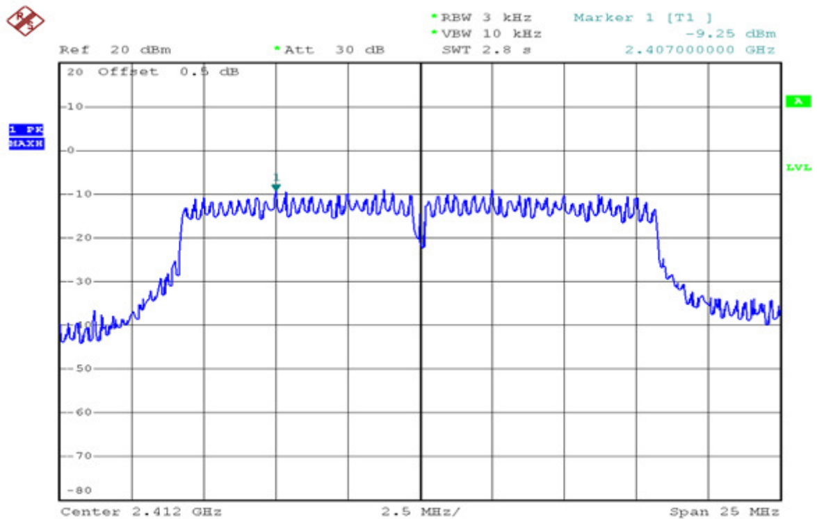
Channel 01 (2412MHz)
