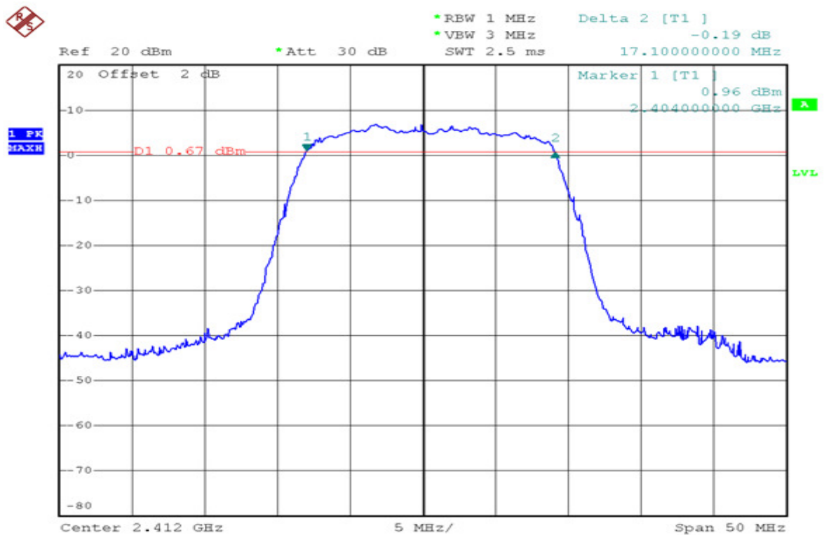
Channel 01 (2412MHz)
