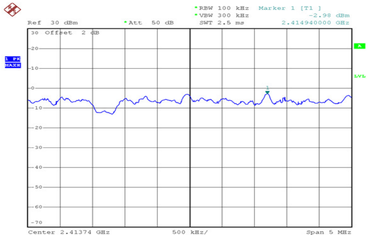
Channel 01 (2412MHz)
