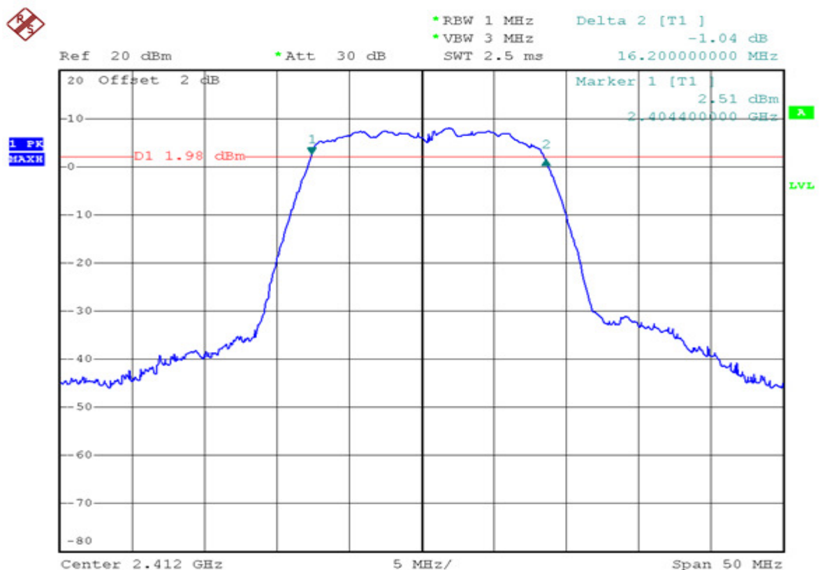
Channel 01 (2412MHz)
