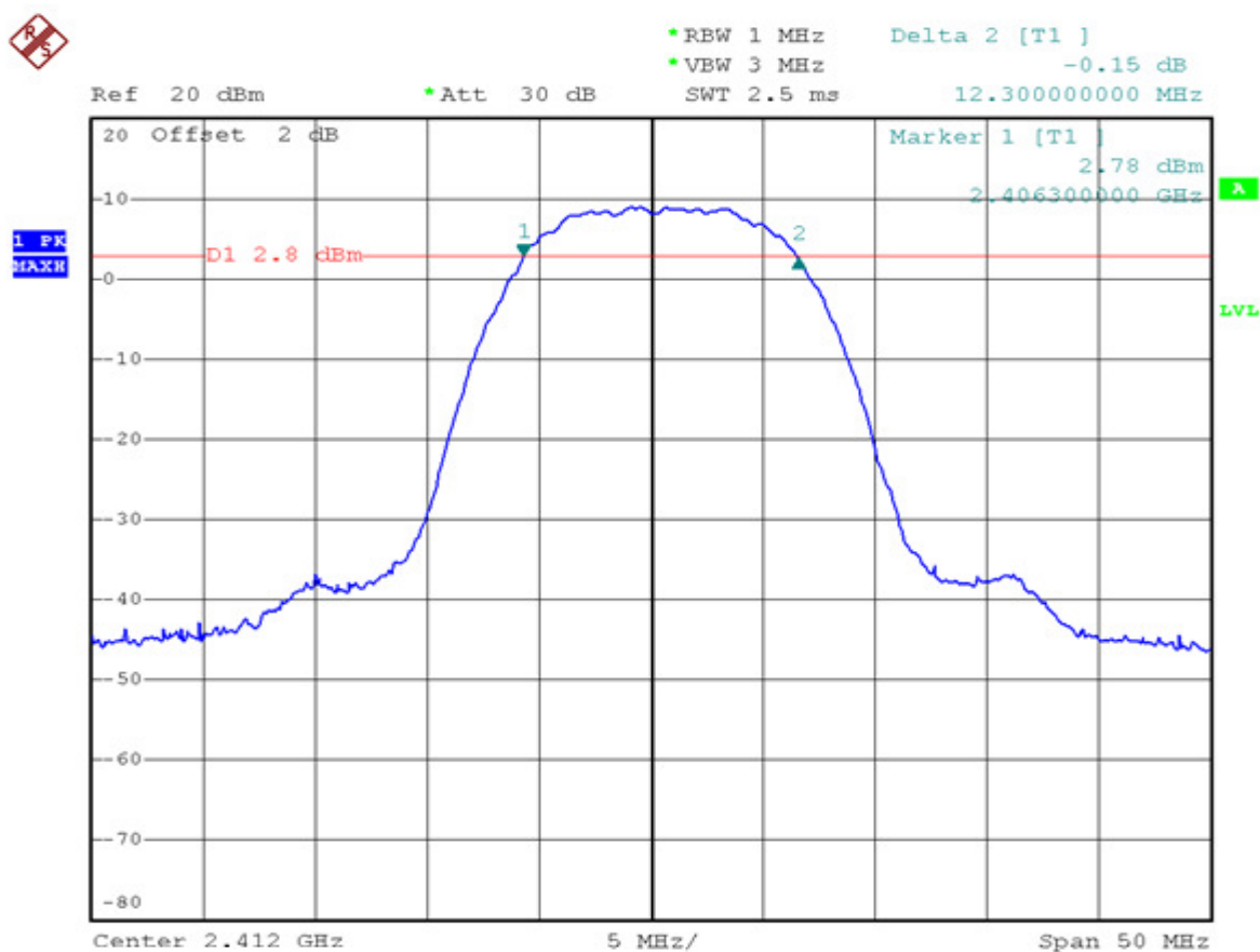
Channel 01 (2412MHz)
