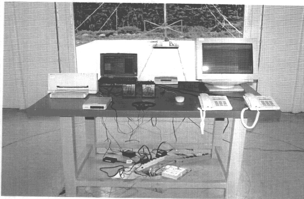
FRONT VIEW OF RADIATED TEST ( Worst Case Test Setup, mode 2)
