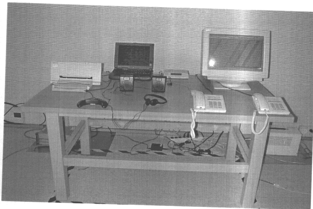
BACK VIEW OF CONDUCTED TEST ( Worst Case Test Setup, mode 1)
