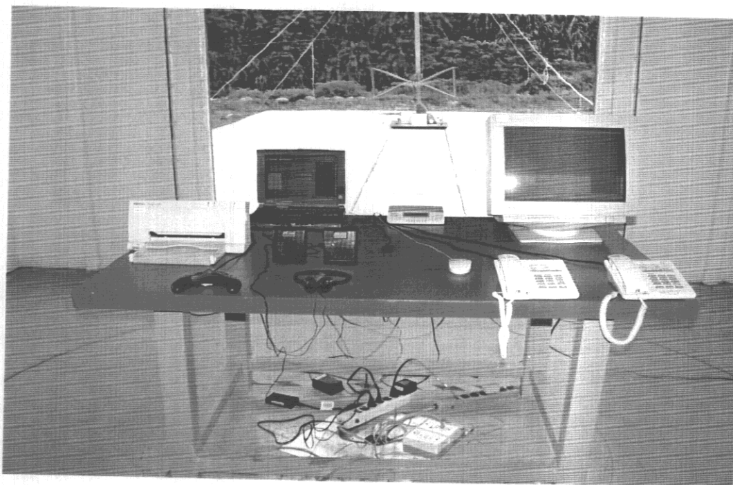
FRONT VIEW OF RADIATED TEST ( Worst Case Test Setup, mode 1)
