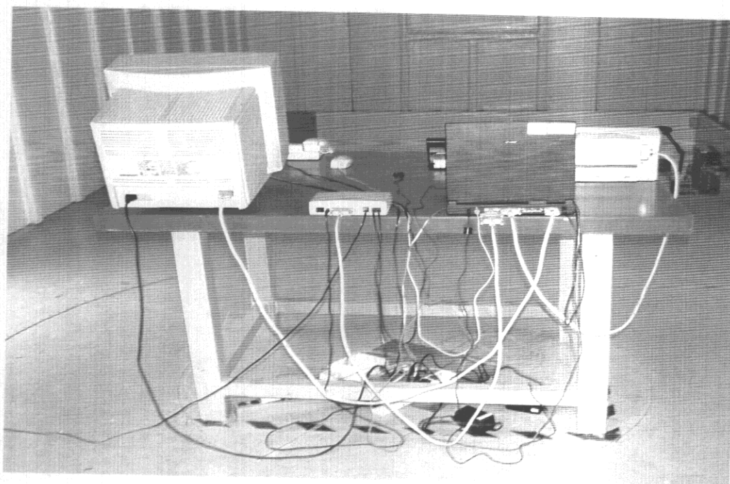
BACK VIEW OF RADIATED TEST ( Worst Case Test Setup, mode 1)
