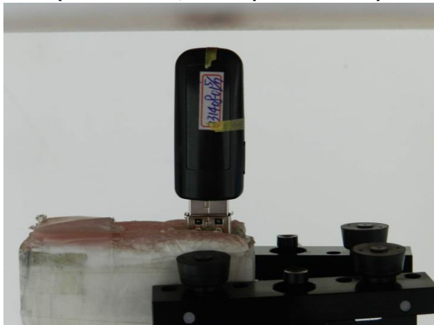
Direct Laptop Plug-in for USB Configuration 5 (Tip Mode, Test Separation 5 mm)
