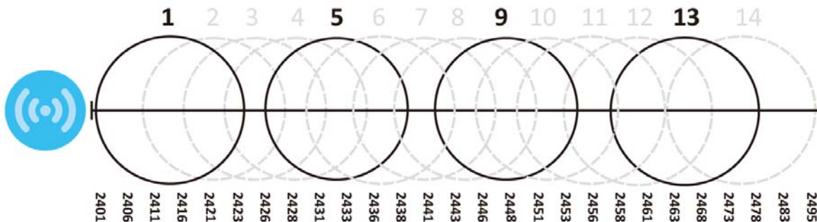
Figure 60 An Alternative Four-Channel Deployment
