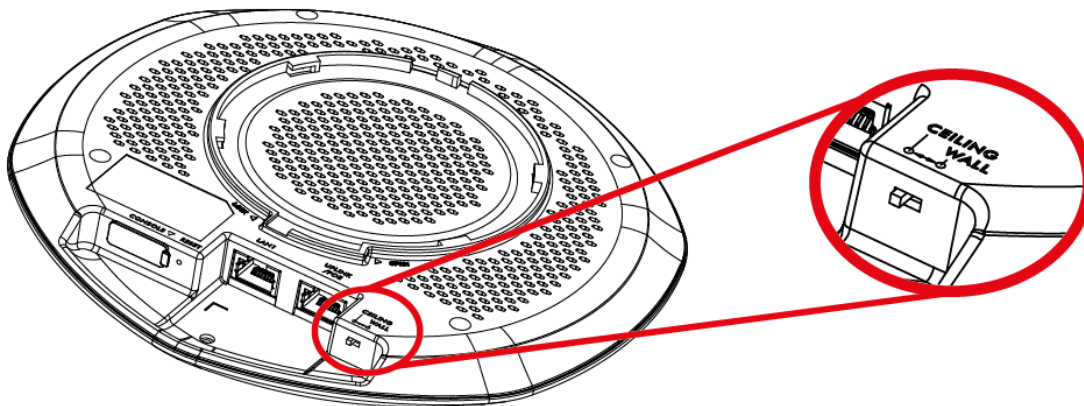
Figure 125 WAC6103D-I Physical Antenna Switch
