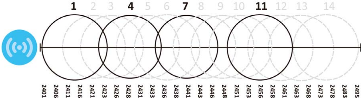
Figure 59 An Example Four-Channel Deployment
