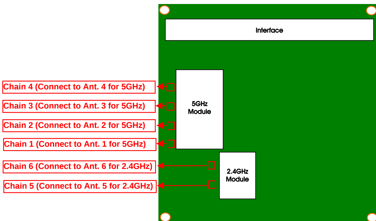
PCB board
