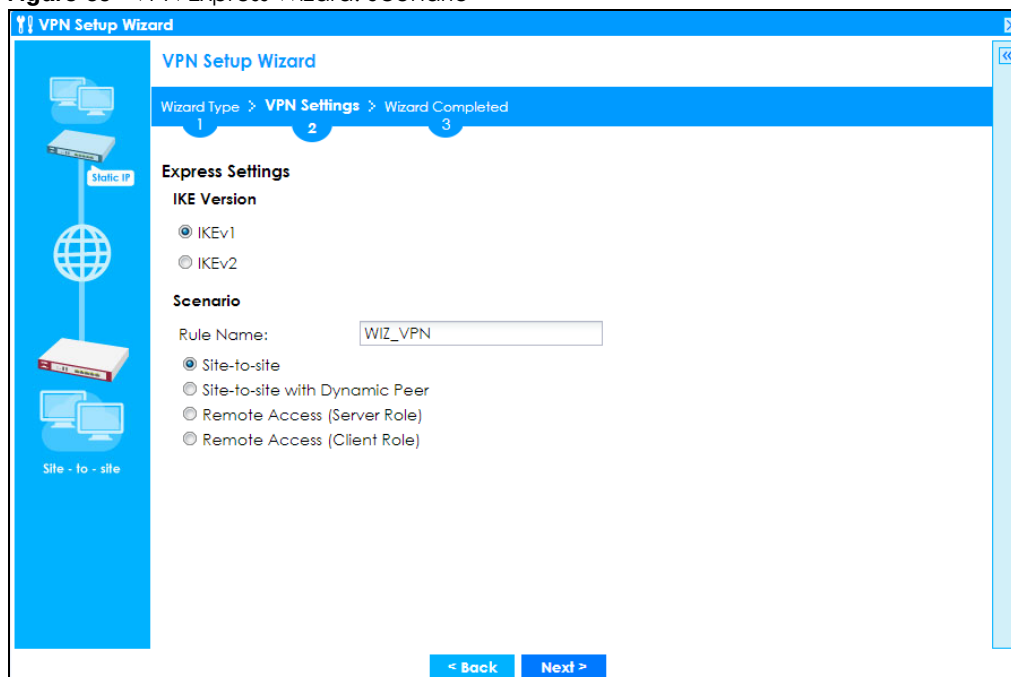
Figure 69 VPN Express Wizard: Scenario
