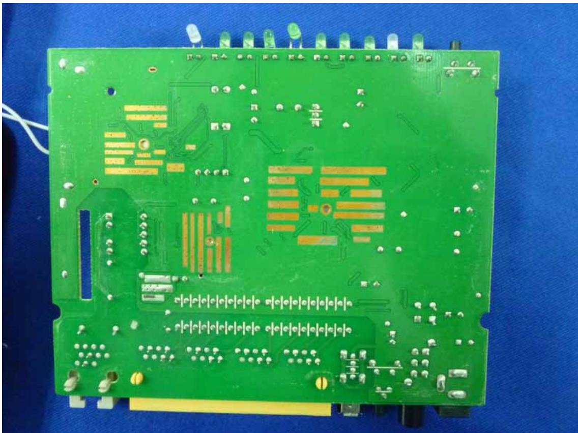
Figure 10 Backside of the PCB
