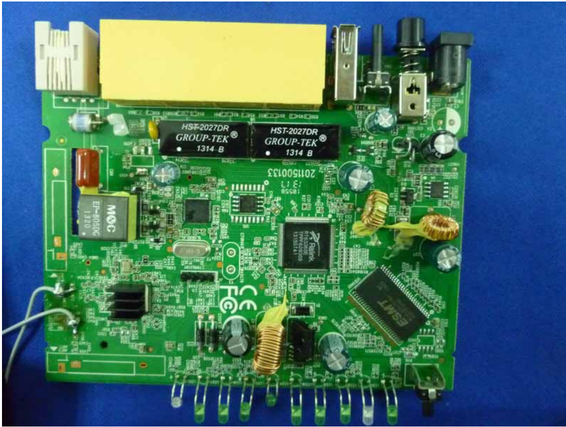
Figure 9 Frontside of the PCB
