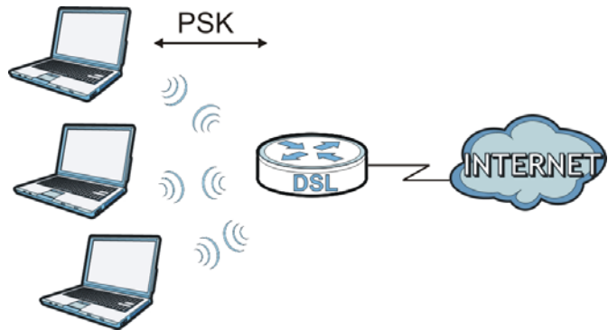
Figure 178 WPA(2)-PSK Authentication
