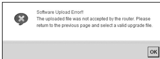
Figure 112 Error Message
