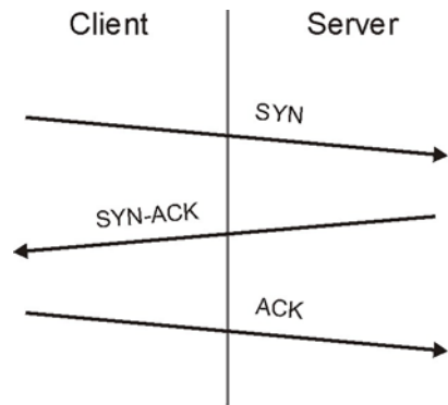
Figure 89 Three-Way Handshake
