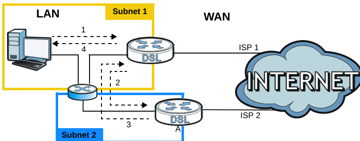
Figure 93 IP Alias
