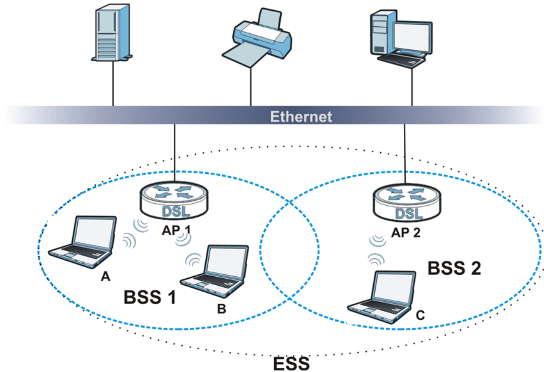
Figure 175 Infrastructure WLAN
