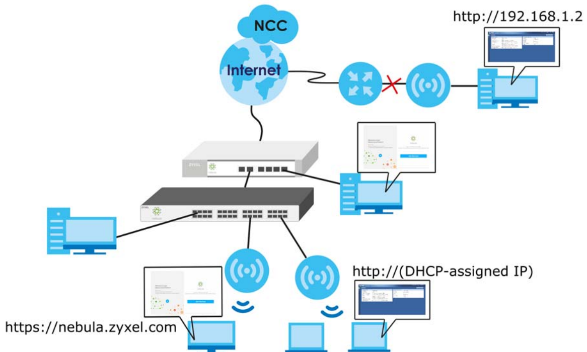
Figure 159 Cloud Mode Application
