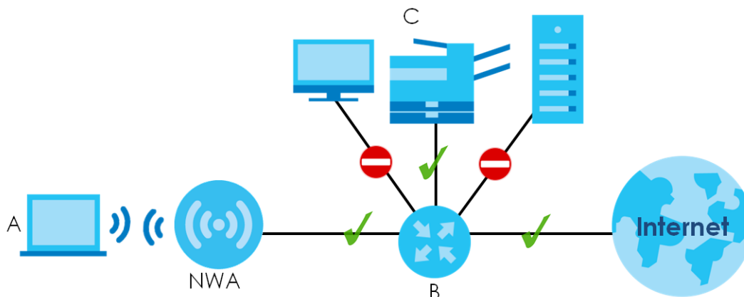
Figure 104 Layer-2 Isolation Application
