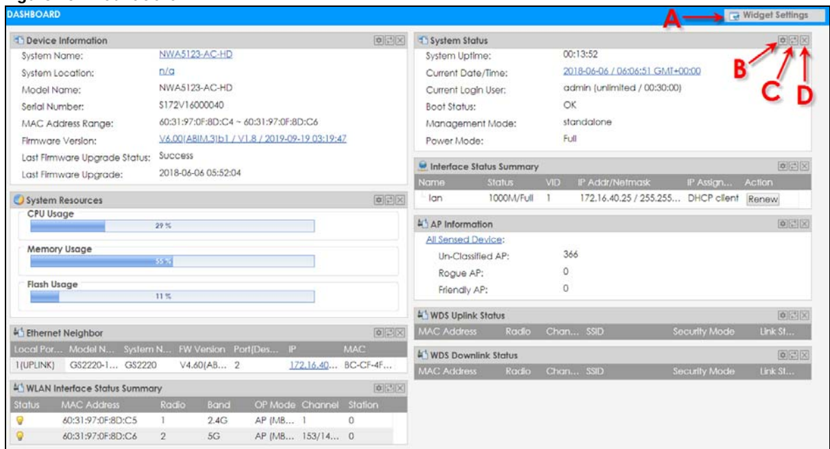
Figure 29 Dashboard
