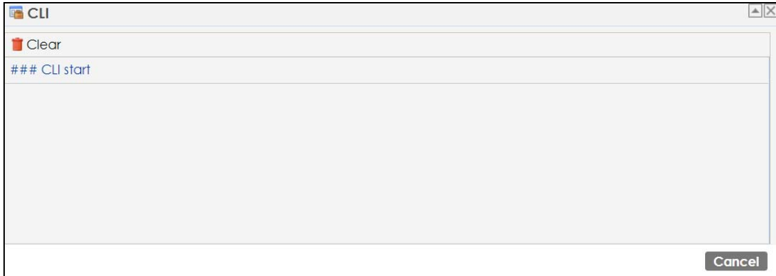
Figure 27 CLI Messages
