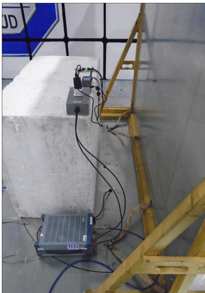
Figure 5 - AC Line Conducted Emissions
