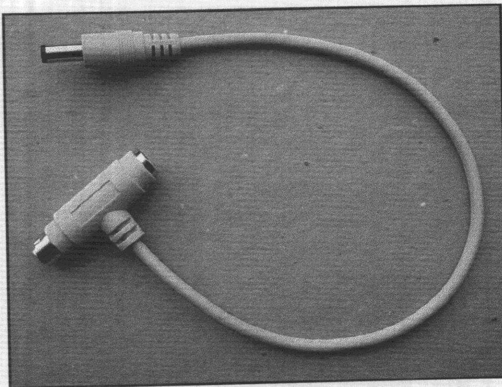
7.8 Power DC cable for derived 5VDC from PS/2 mouse or keyboard port
