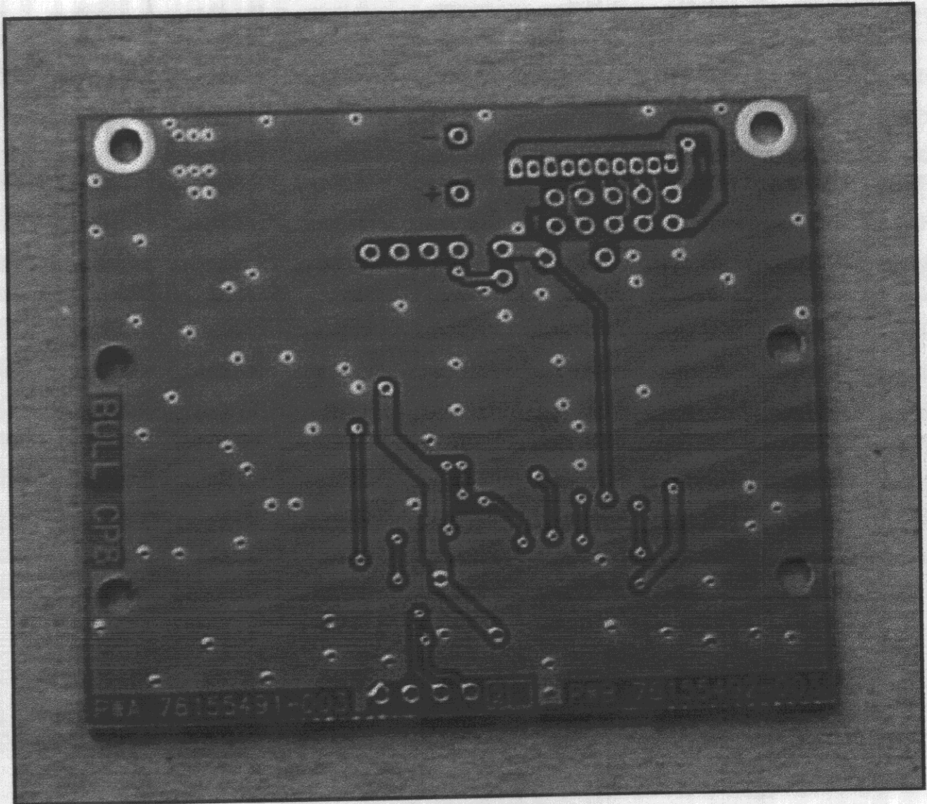
7.7 Solder side board
