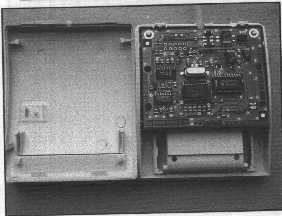
7.3 SmarTLP3 with upper cover removed
