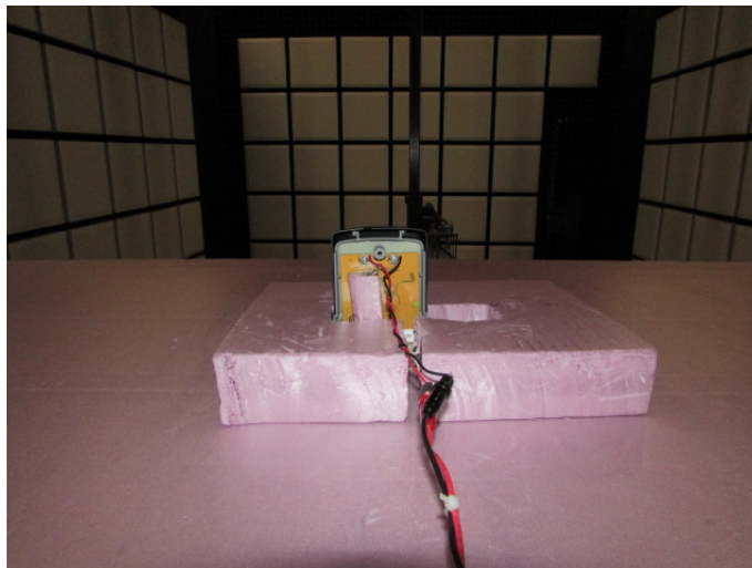
Figure 4: Radiated Spurious Emissions Test Setup – Rear View
