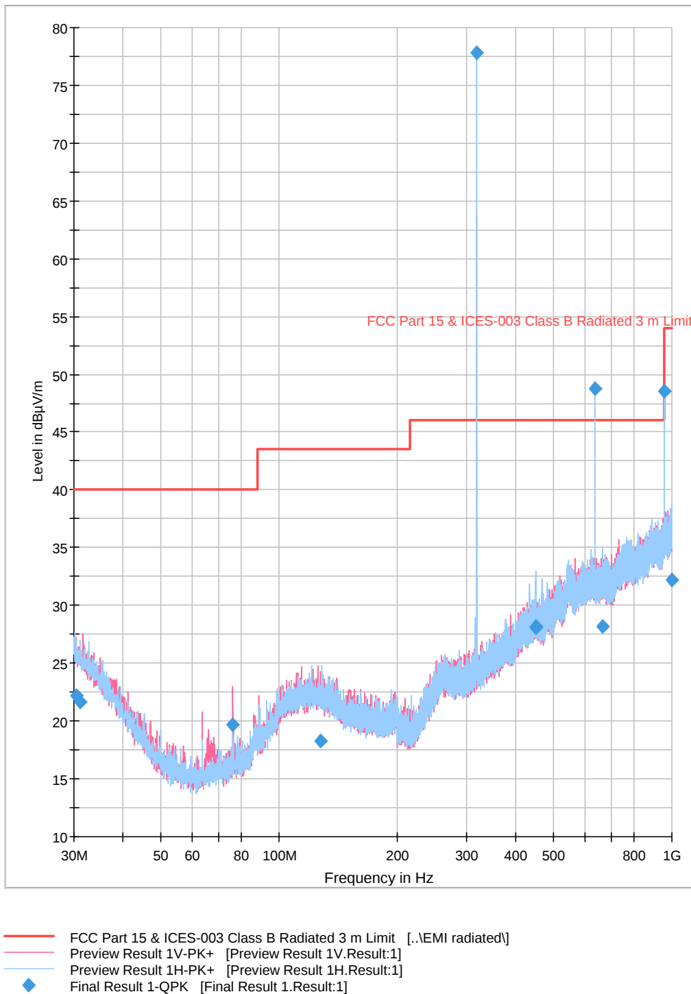
Figure 2.2.9-1 – Radiated Emissions Plot 30 MHz – 1 GHz
