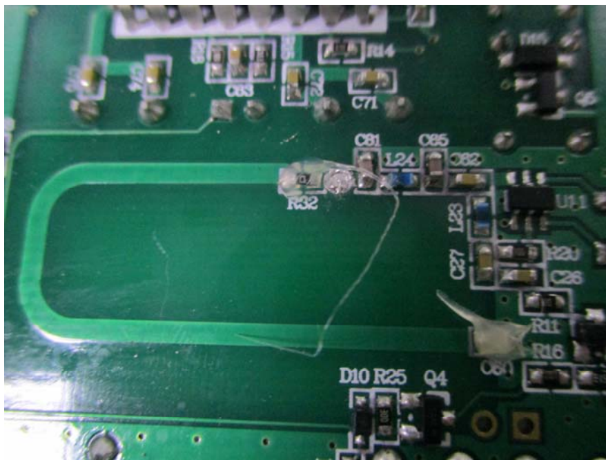
EUT –318MHz Antenna View
