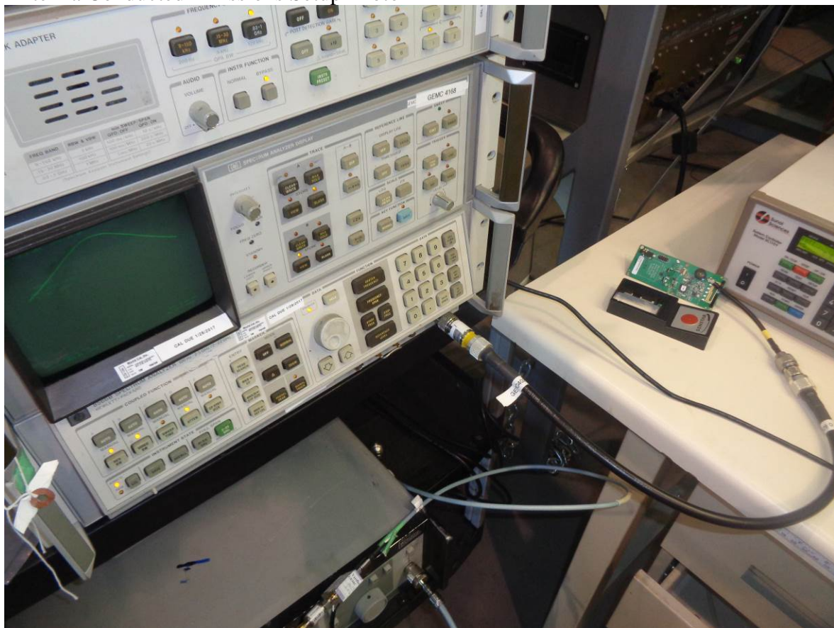
Antenna Conducted Emissions Setup Photo
