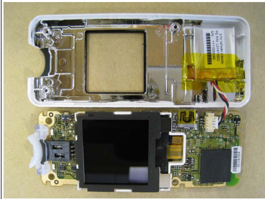
PCB BACK
