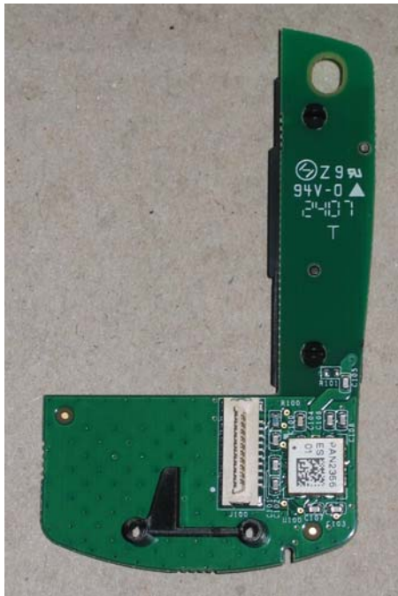
RF Board component side
