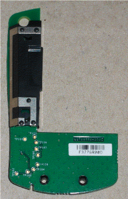
RF Board antenna side
