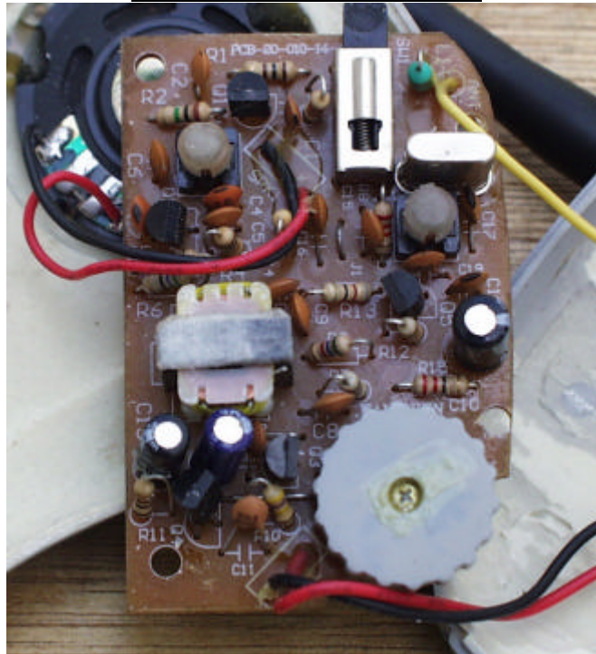
INNER CIRCUIT BOTTOM VIEW
