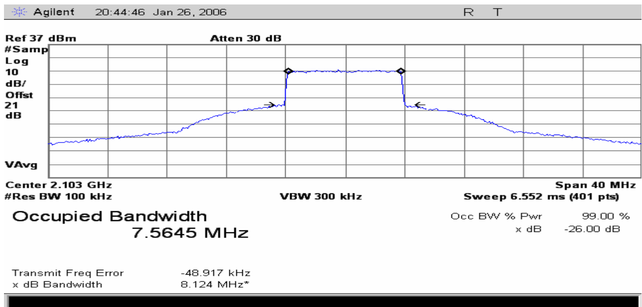
Figure 36 Occupied Bandwidth measurement; Modulation overlaying Mask and measured Power Bandwidth. COFDM modulation, 8 MHz 16QAM, Color Bars with Audio
