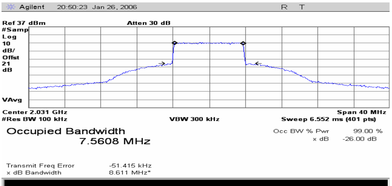
Figure 33 Occupied Bandwidth measurement; Modulation overlaying Mask and measured Power Bandwidth. COFDM modulation, 8 MHz 16QAM color Bars with Audio
