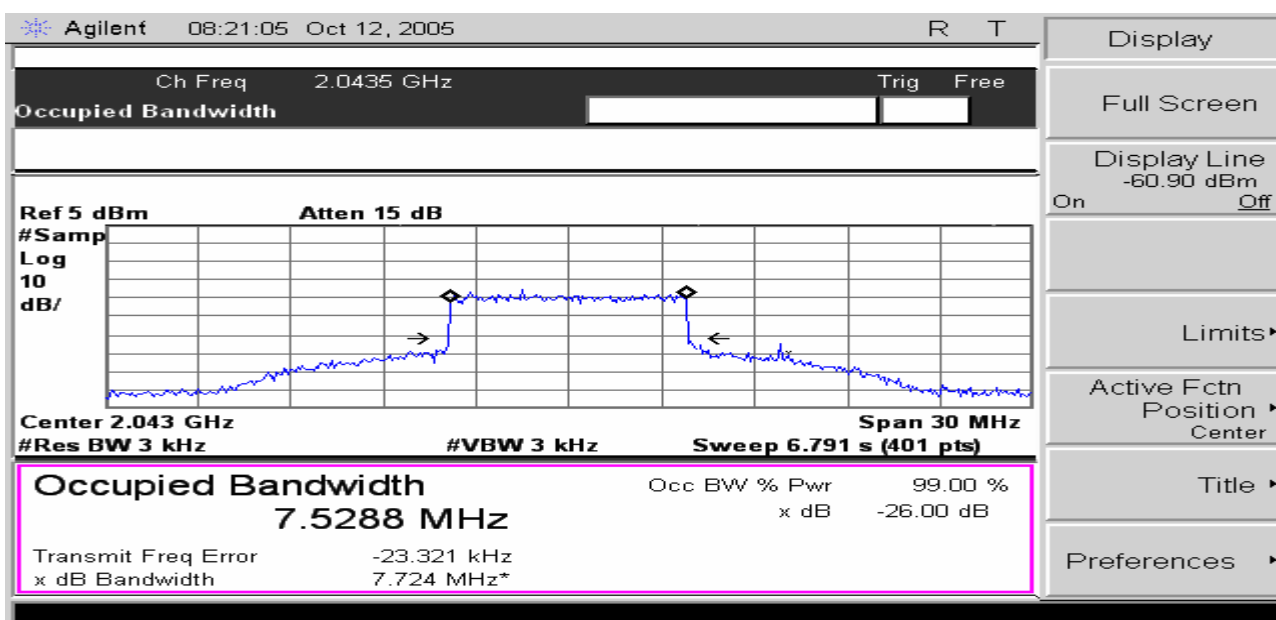
Figure 34 Occupied Bandwidth measurement; Modulation overlaying Mask and measured Power Bandwidth. COFDM modulation, 8 MHz 16 QAM, Color Bars with Audio
