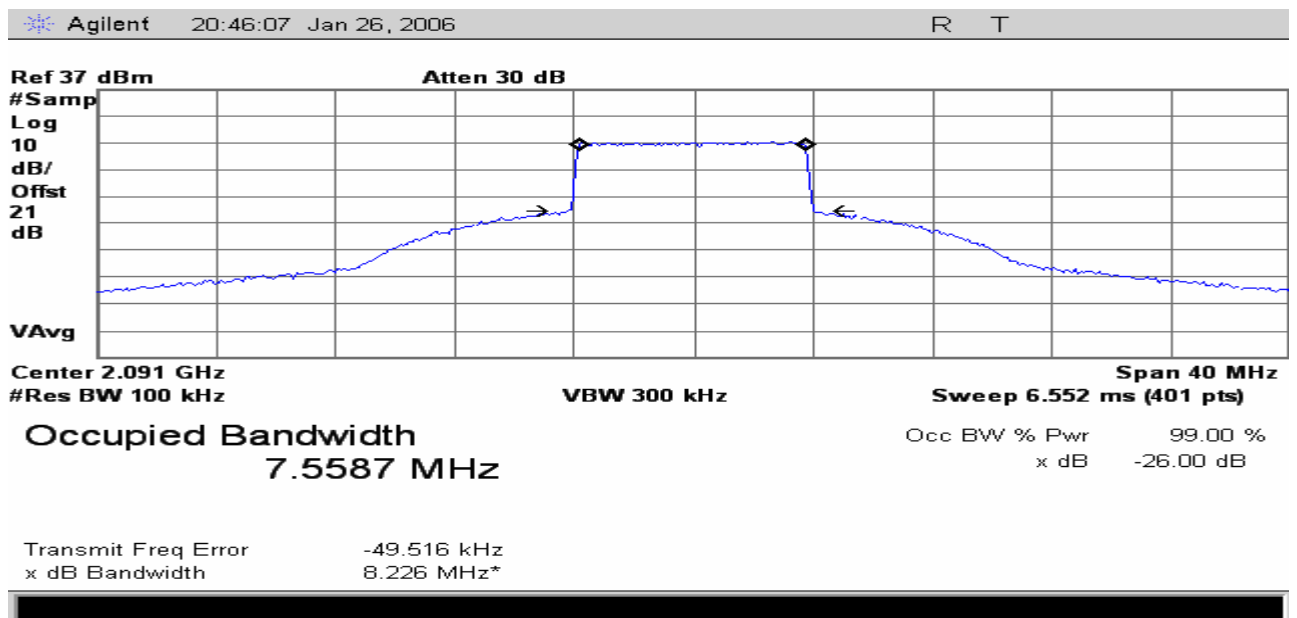
Figure 35 Occupied Bandwidth measurement; Modulation overlaying Mask and measured Power Bandwidth. COFDM modulation, 8 MHz 16QAM, Color Bars with Audio
