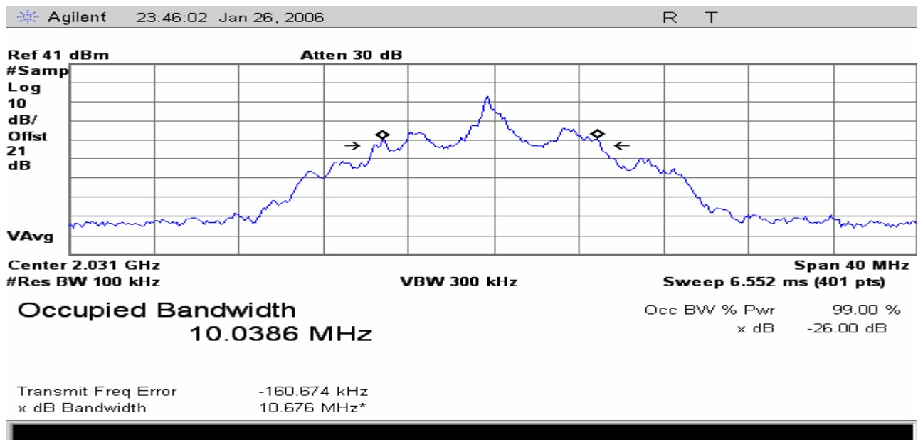
Figure 37 Occupied Bandwidth measurement; Modulation overlaying Mask and measured Power Bandwidth. FM , +/- 3 MHz Deviation ,Color Bars with Audio
