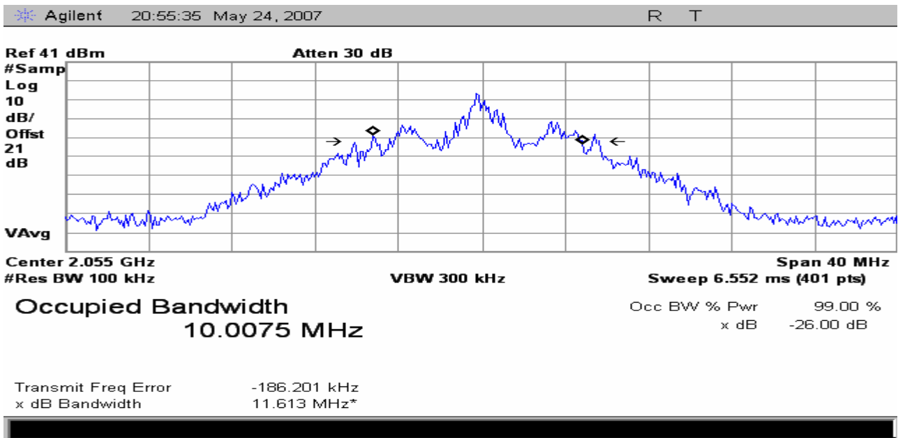
Figure 6 Occupied Bandwidth measurement; Modulation overlaying Mask and measured Power Bandwidth. FM , +/- 3 MHz Deviation ,Color Bars with Audio Channel 3 BAS relo frequency
