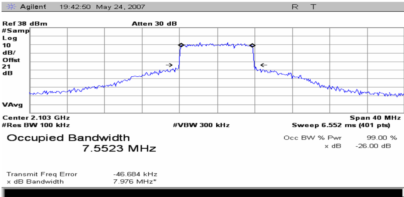
Figure 4 Occupied Bandwidth measurement; Modulation overlaying Mask and measured Power Bandwidth. COFDM modulation, 8 MHz 16QAM, Color Bars with Audio
