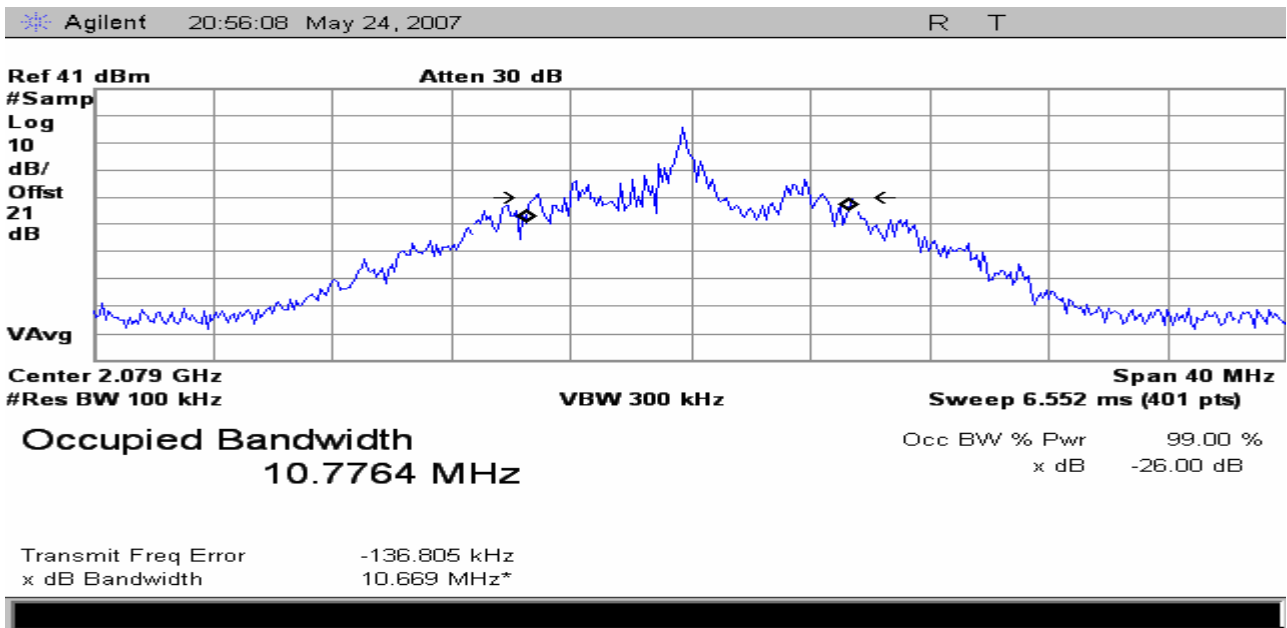
Figure 7 Occupied Bandwidth measurement; Modulation overlaying Mask and measured Power Bandwidth. FM , +/- 3 MHz Deviation ,Color Bars with Audio Channel 5 BAS relo frequency
