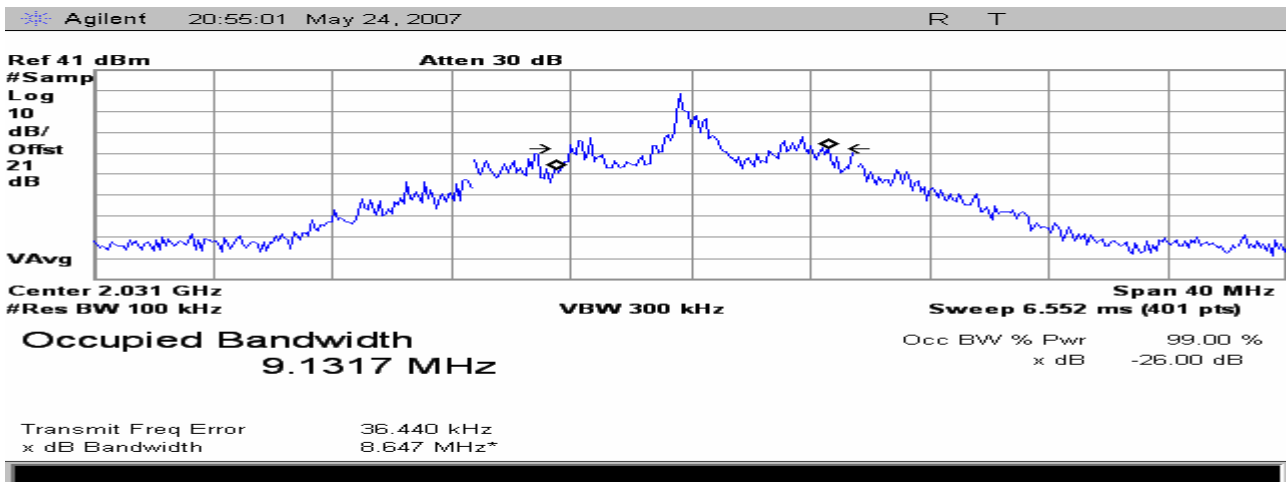
Figure 5 Occupied Bandwidth measurement; Modulation overlaying Mask and measured Power Bandwidth. FM , +/- 3 MHz Deviation ,Color Bars with Audio
