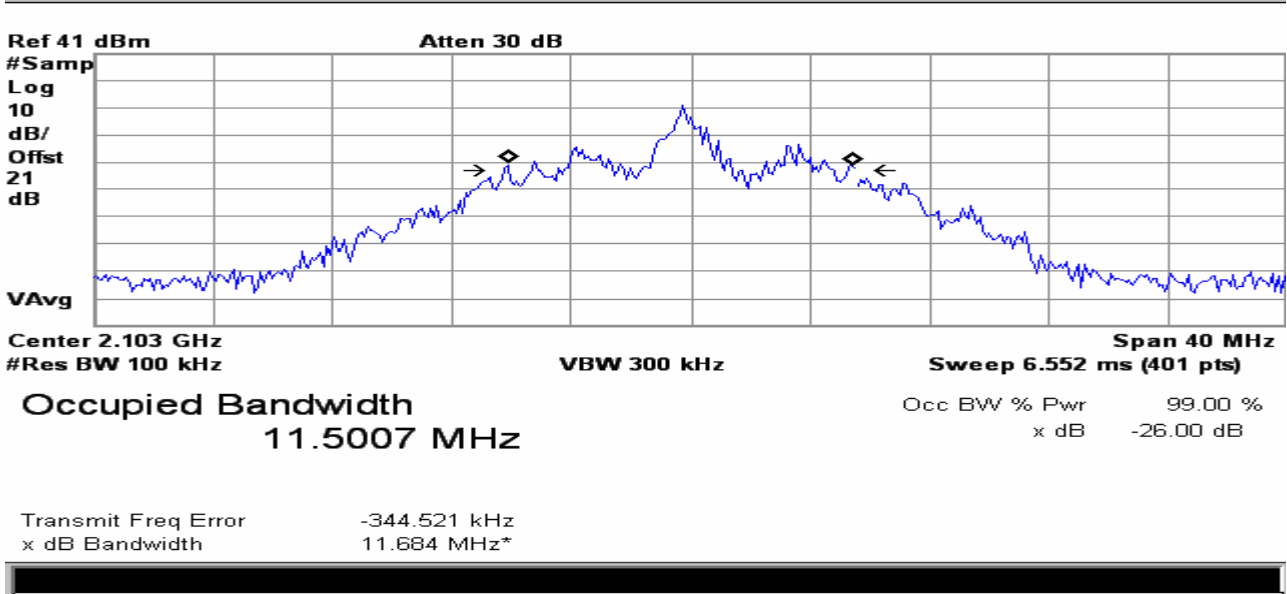
Figure 8 Occupied Bandwidth measurement; Modulation overlaying Mask and measured Power Bandwidth. FM , +/- 3 MHz Deviation ,Color Bars with Audio Channel 7 BAS relo frequency
