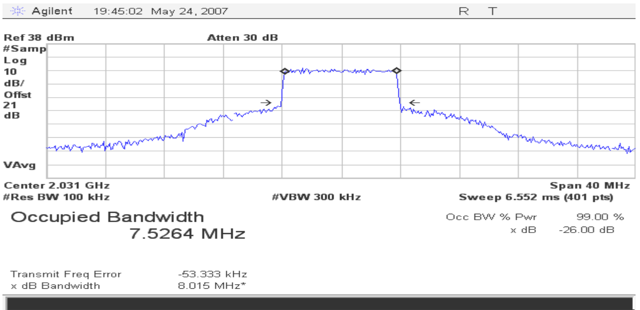
Figure 1 Occupied Bandwidth measurement; Modulation overlaying Mask and measured Power Bandwidth. COFDM modulation, 8 MHz 16QAM color Bars with Audio
