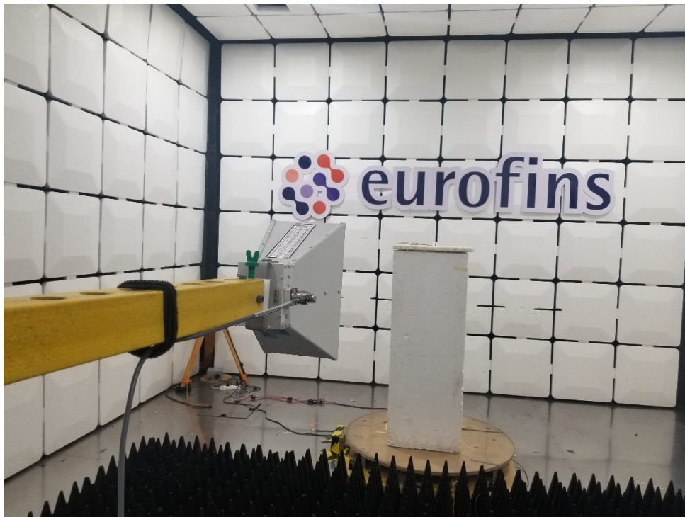
Picture 1 Radiated Spurious Emissions Test Setup
