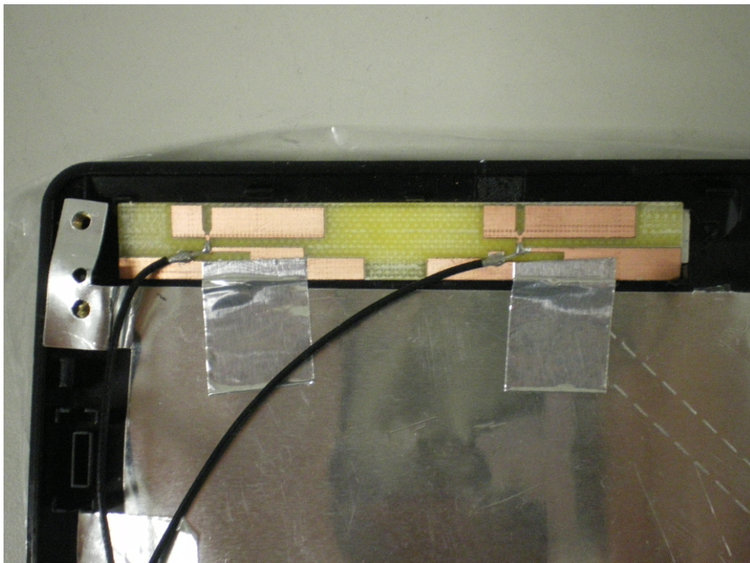
(10) EUT Photo (JI-HAW for WLAN Antenna)
