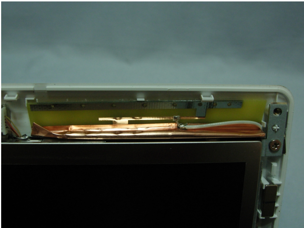
(8) EUT Photo (WWAN Antenna)
