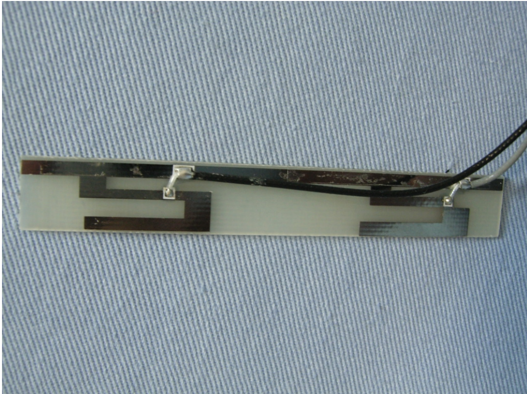
(7) EUT Photo (JOINSOON for WLAN Antenna)
