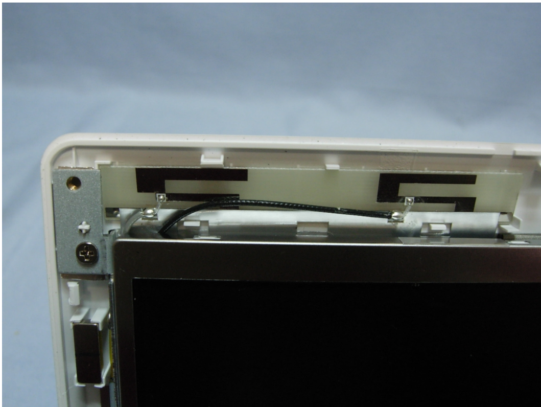
(6) EUT Photo (JOINSOON for WLAN Antenna)
