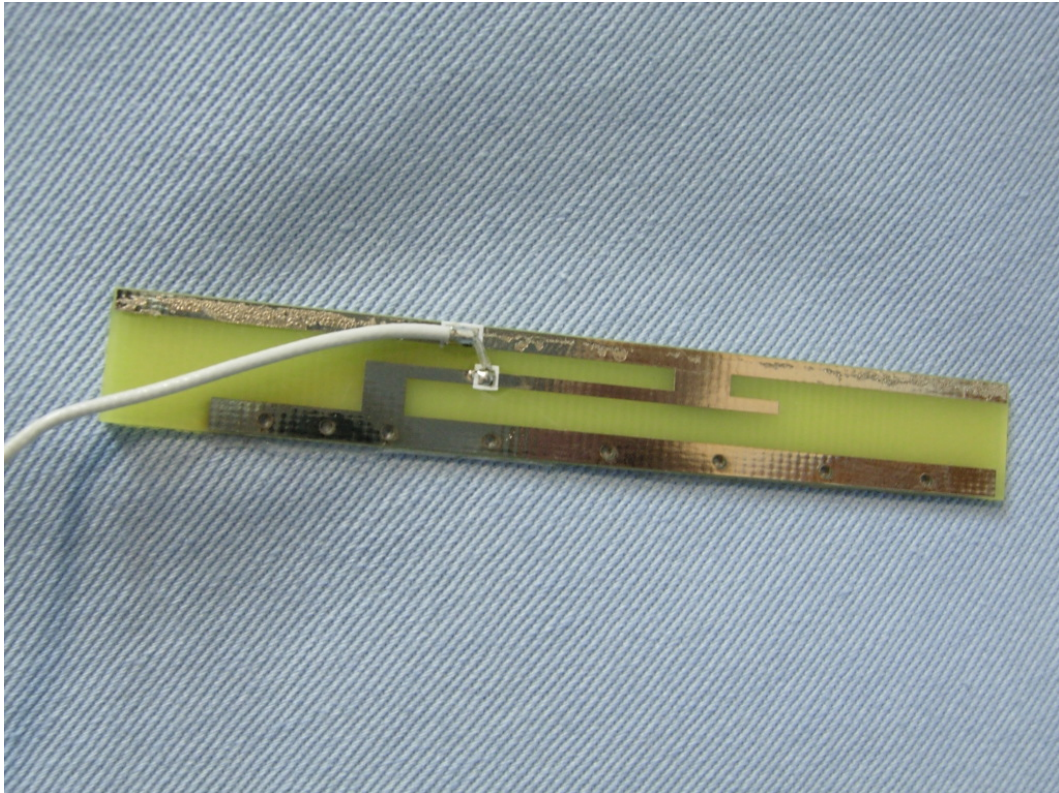
(9) EUT Photo (WWAN Antenna)
