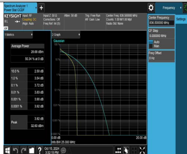
Band26-1.4MHz-QPSK-26915-1RB#0
