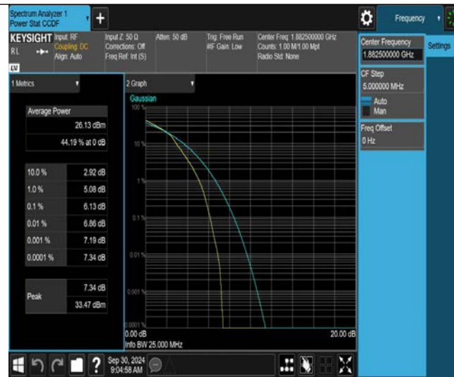
Band25-5MHz-16QAM-26665-1RB#0
