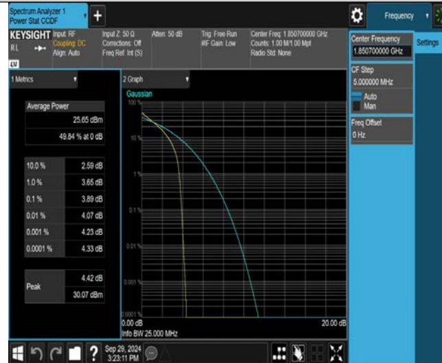
Band25-1.4MHz-QPSK-26047-6RB#0
