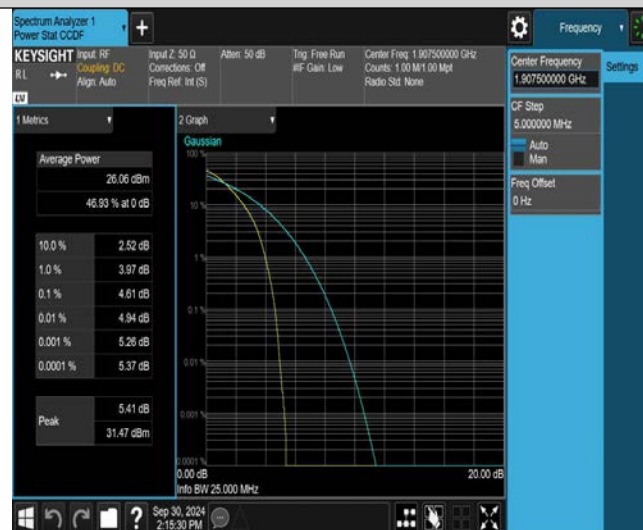
Band25-15MHz-16QAM-26115-1RB#0
