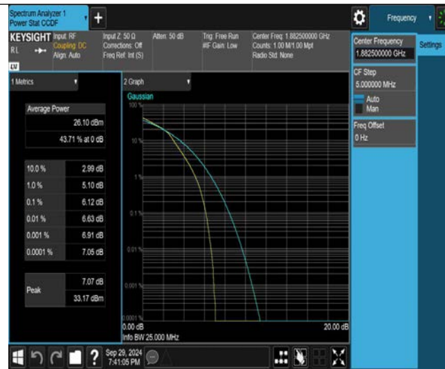
Band25-3MHz-16QAM-26675-1RB#0
