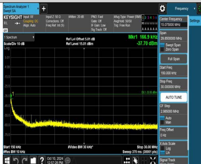
Band2-9400-4-0.15~30MHz
