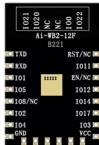
Figure 6 Schematic diagram of module pins
