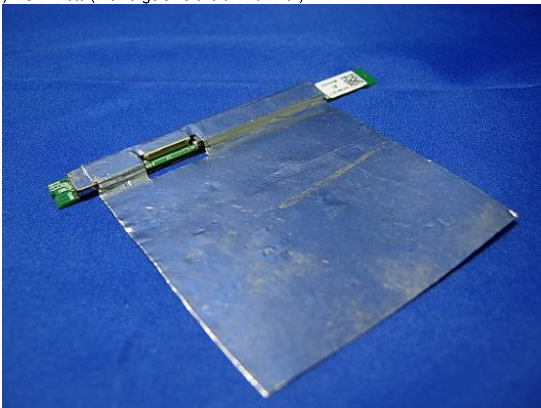
(8) EUT Photo (with large size of aluminum foil)
