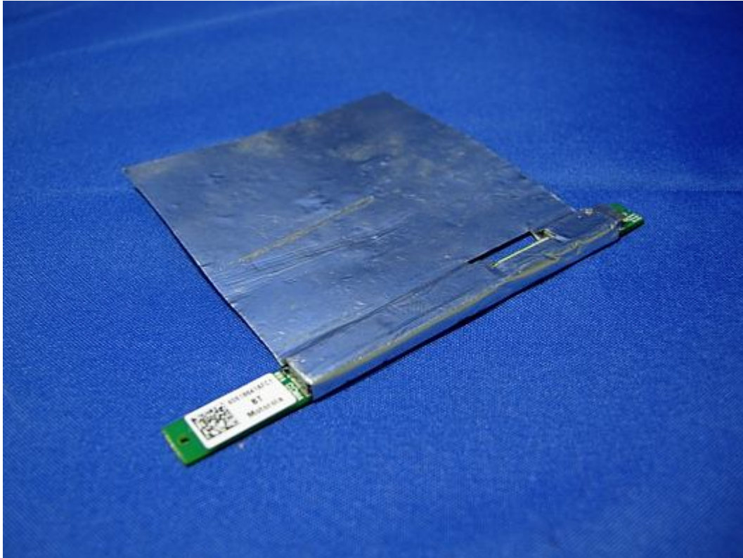
(10) EUT Photo (with large size of aluminum foil)
