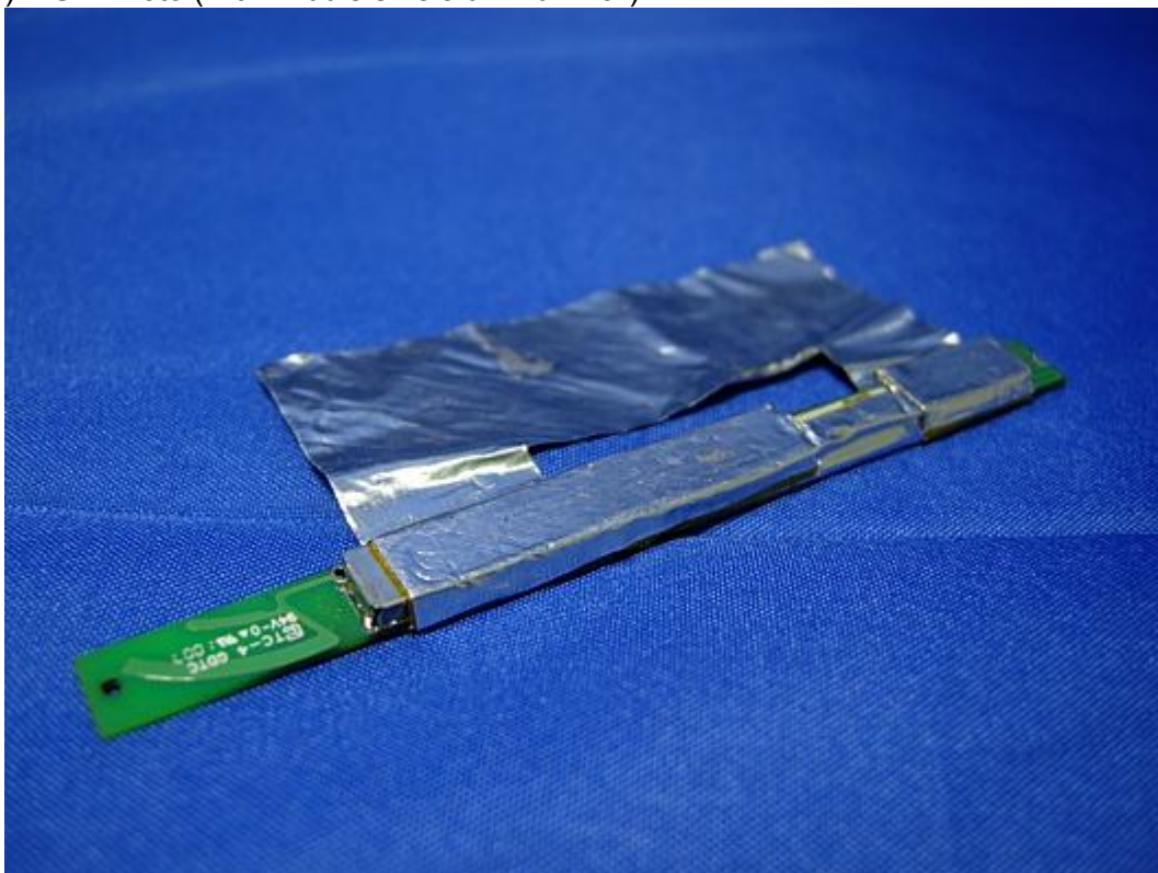
(6) EUT Photo (with middle size aluminum foil)
