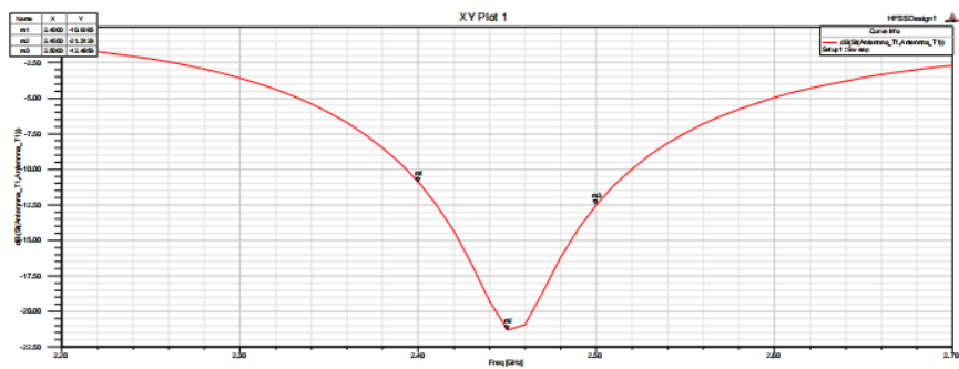
Figure 8 shows S11 figure.
