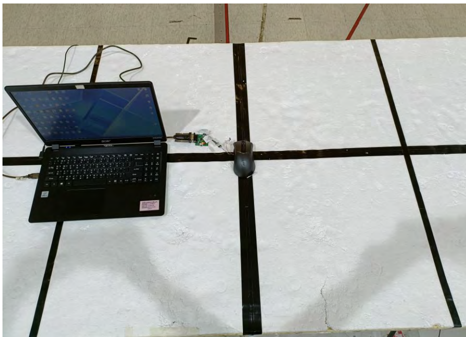
Below 1 GHz _ Rear View
