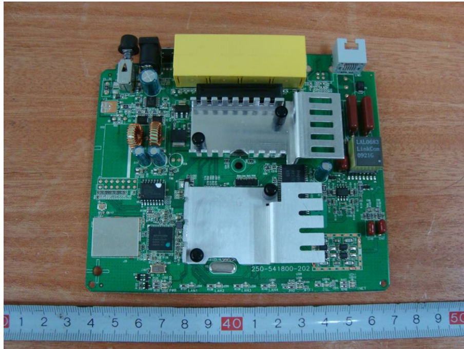
EUT – Main Board With Shielded Cover and Heat Sink Top View
