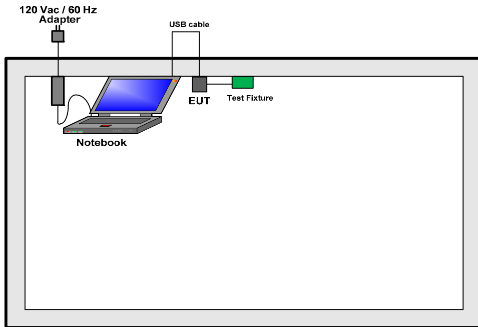
Test Setup Diagram - Radiated Mode 2 (Above 1GHz)
