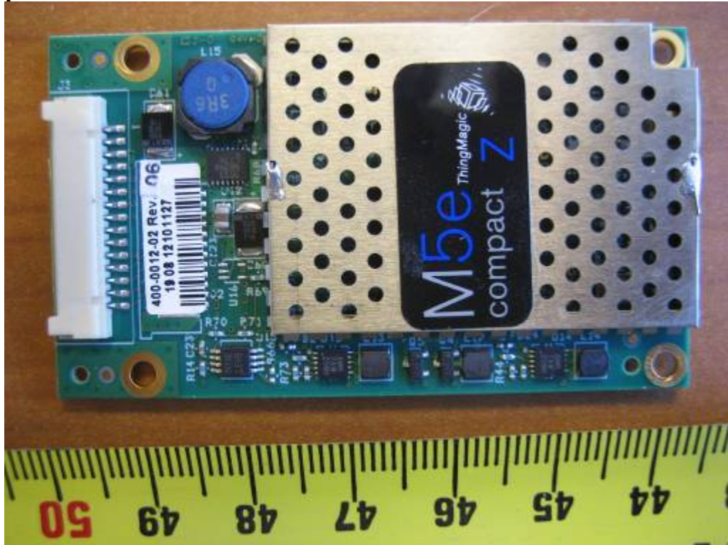
EUT Photo-RFID Radio Component View-1with RF shield
