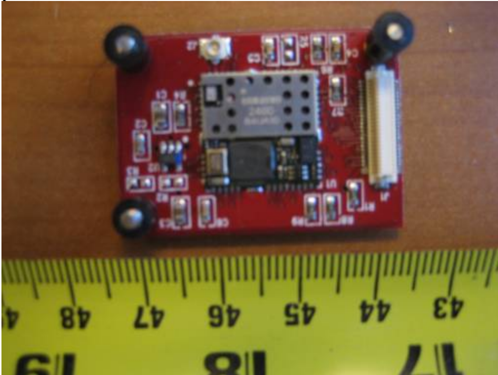
EUT Photo-WLAN Radio Component View-1
