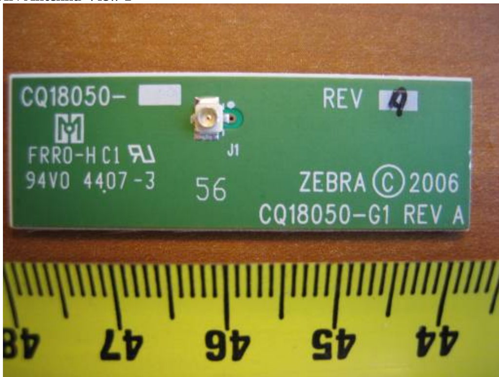
WLAN Antenna-View 1
