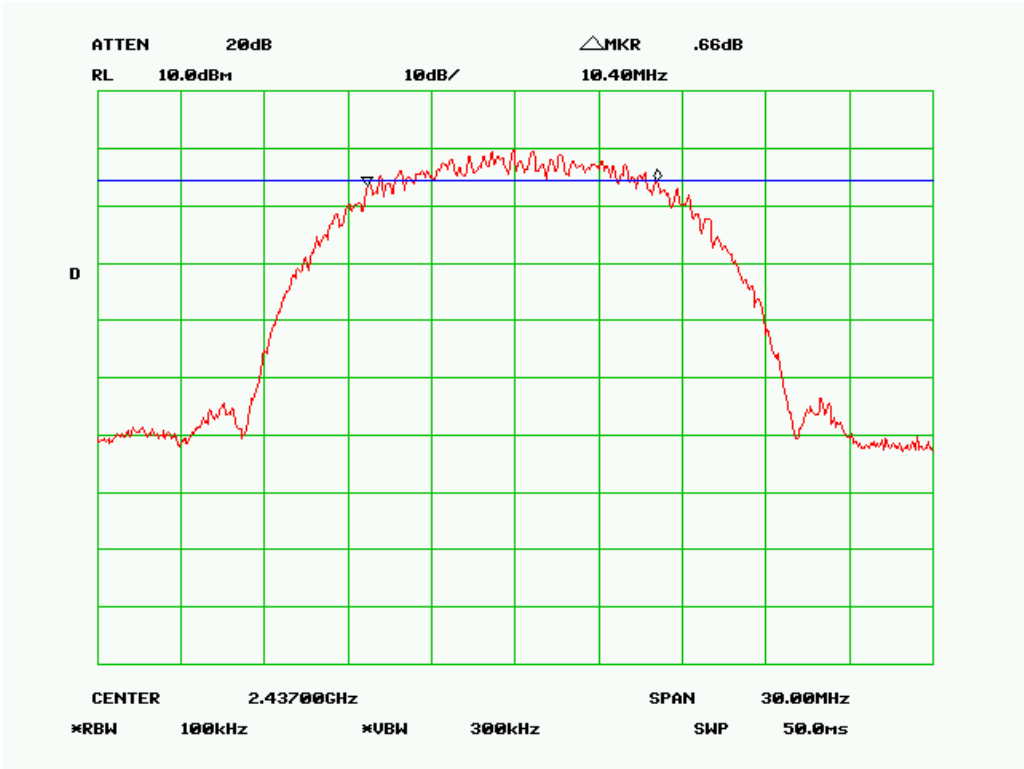
6 dB Bandwidth - 802.11b, Middle Channel
