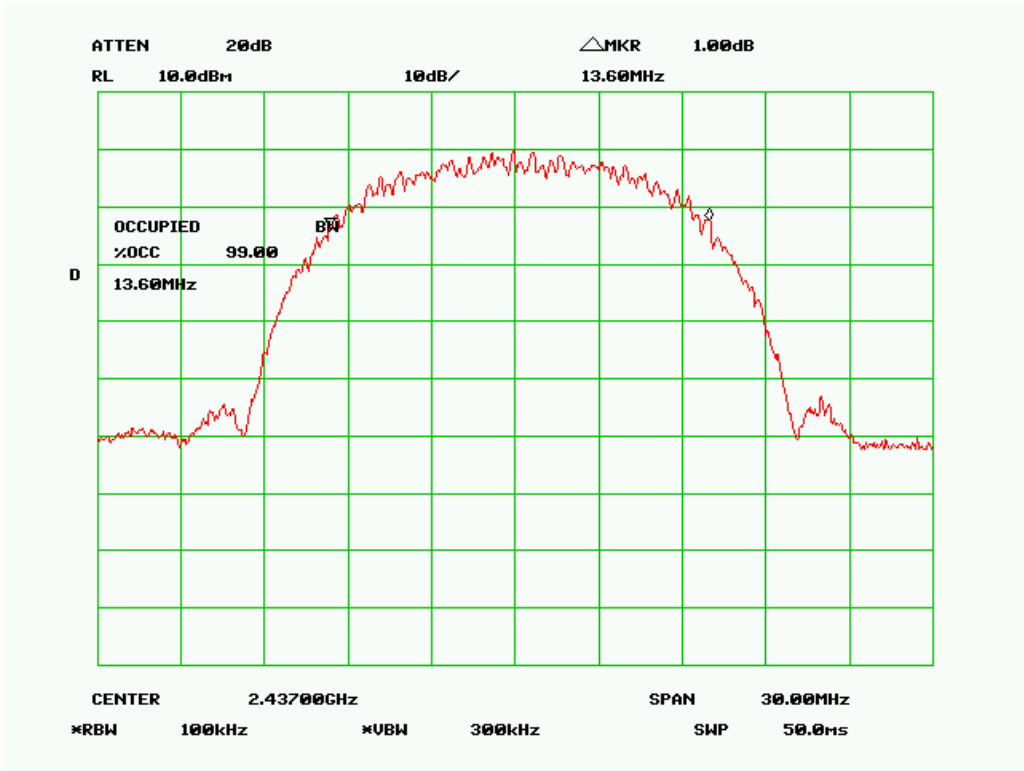
99% dB Bandwidth - 802.11b, Mid Channel
