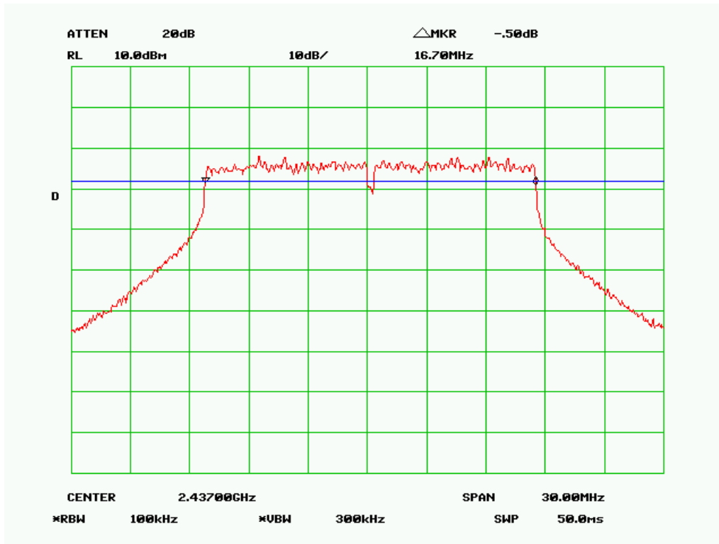
6 dB Bandwidth - 802.11g, Middle Channel
