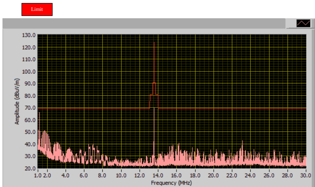
Radiated Emissions Plot
