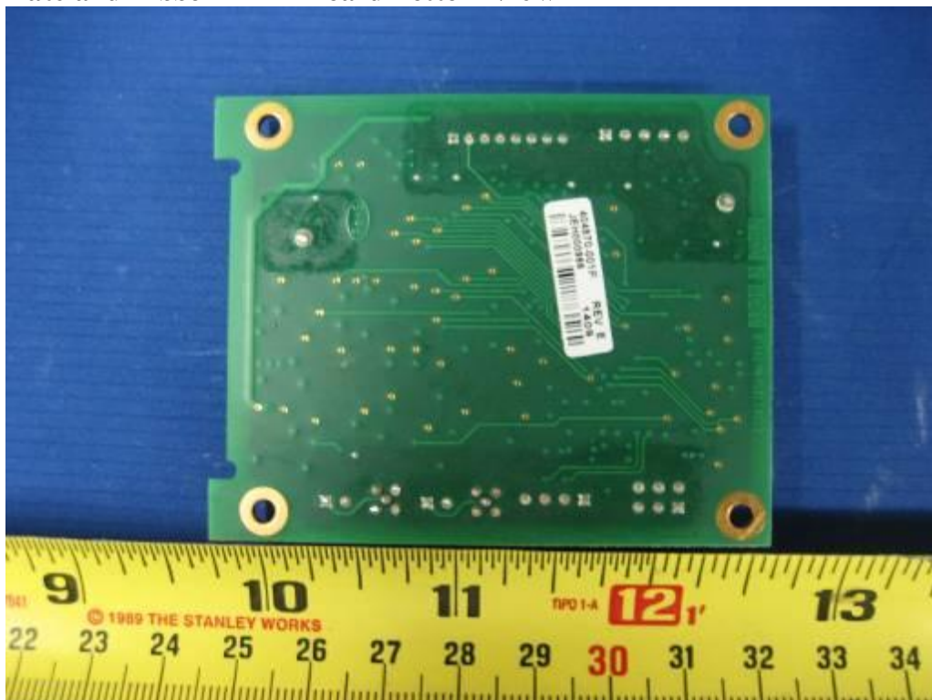
Laminate and Ribbon RFID Board Bottom View
