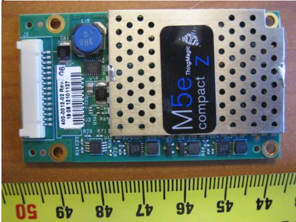
EUT Photo-RFID Component View-1with RF shield
