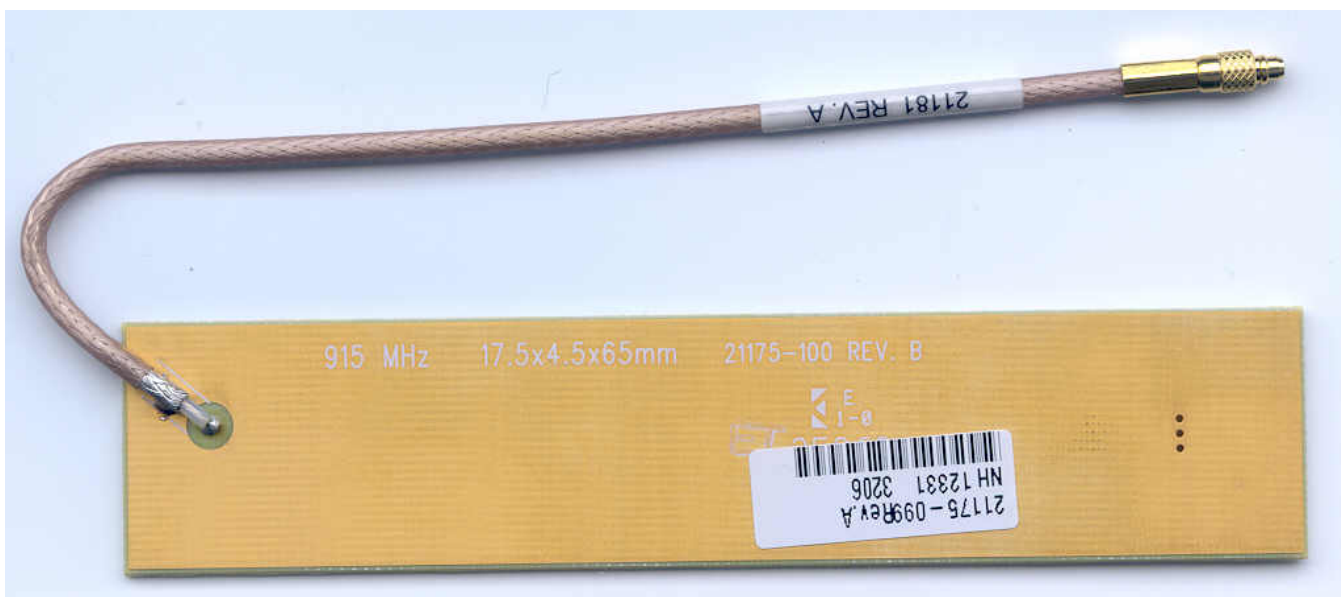
21175-099 GROUND PLANE SIDE
