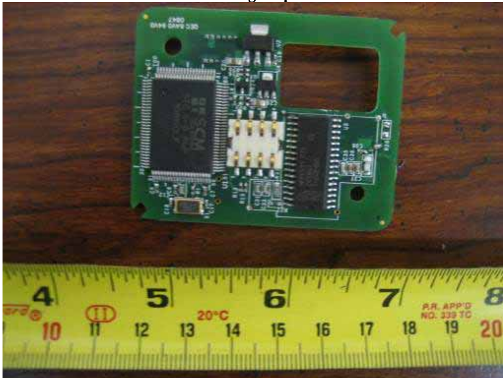
Contactless RFID Board without shielding -Top View
