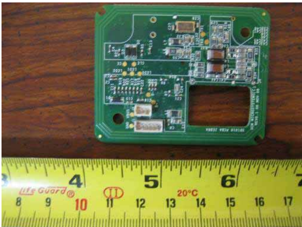
Contactless RFID Board without shielding –Bottom View
