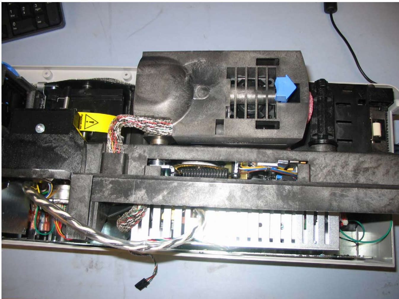
P430i PRINTER
