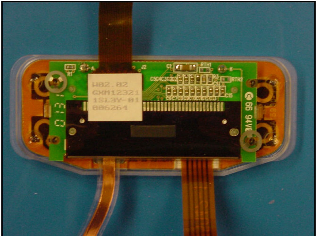
PHOTOGRAPH 11: REAR OF LCD DISPLAY
