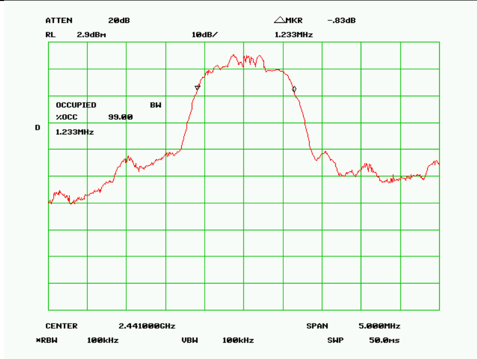
99% dB Bandwidth - Mid Channel
