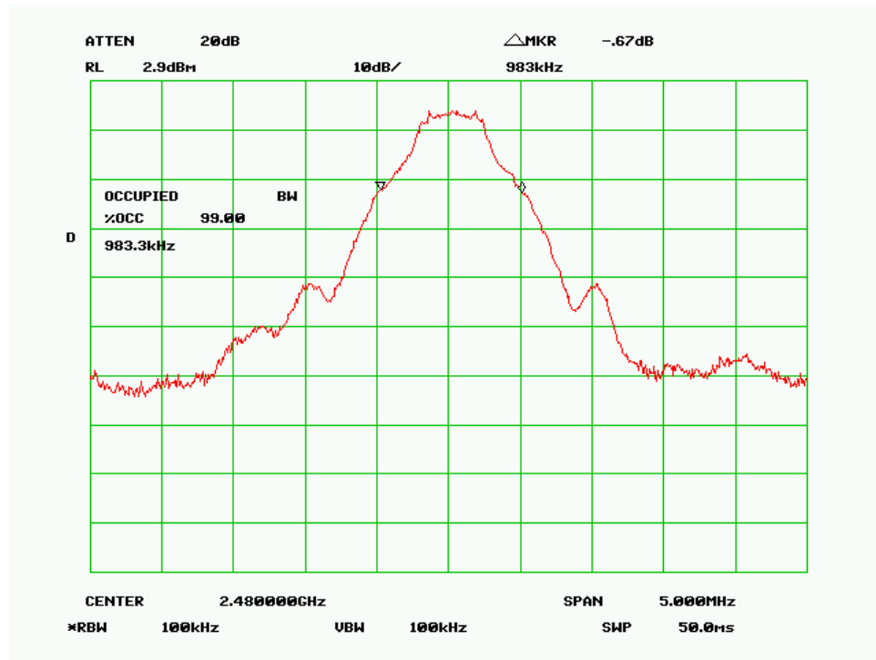
99% dB Bandwidth - High Channel
