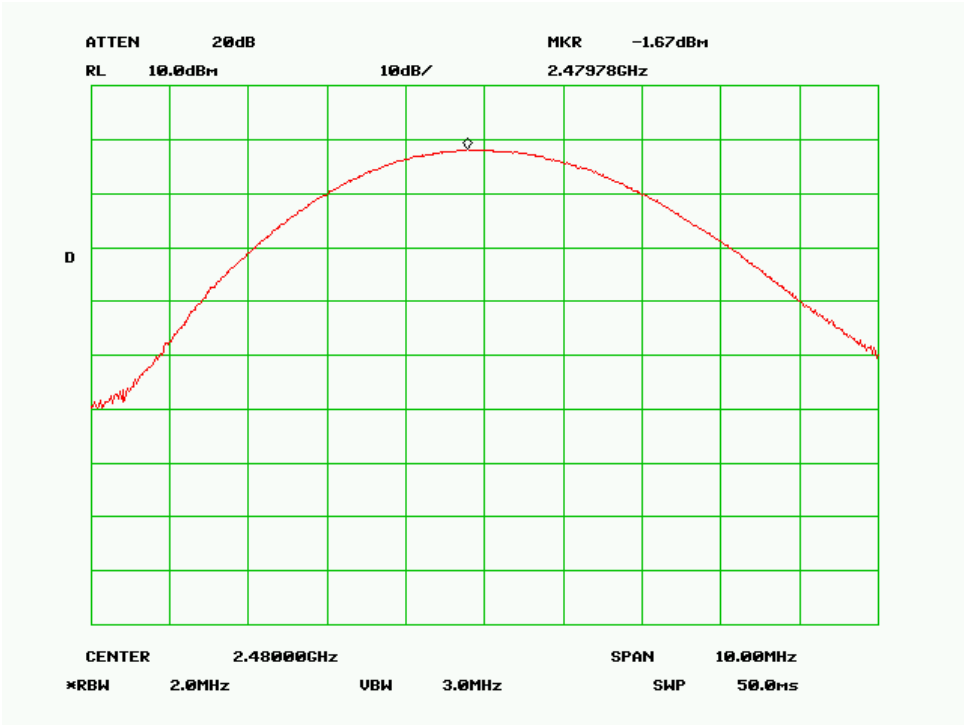
Output Power High Channel (Bluetooth)
