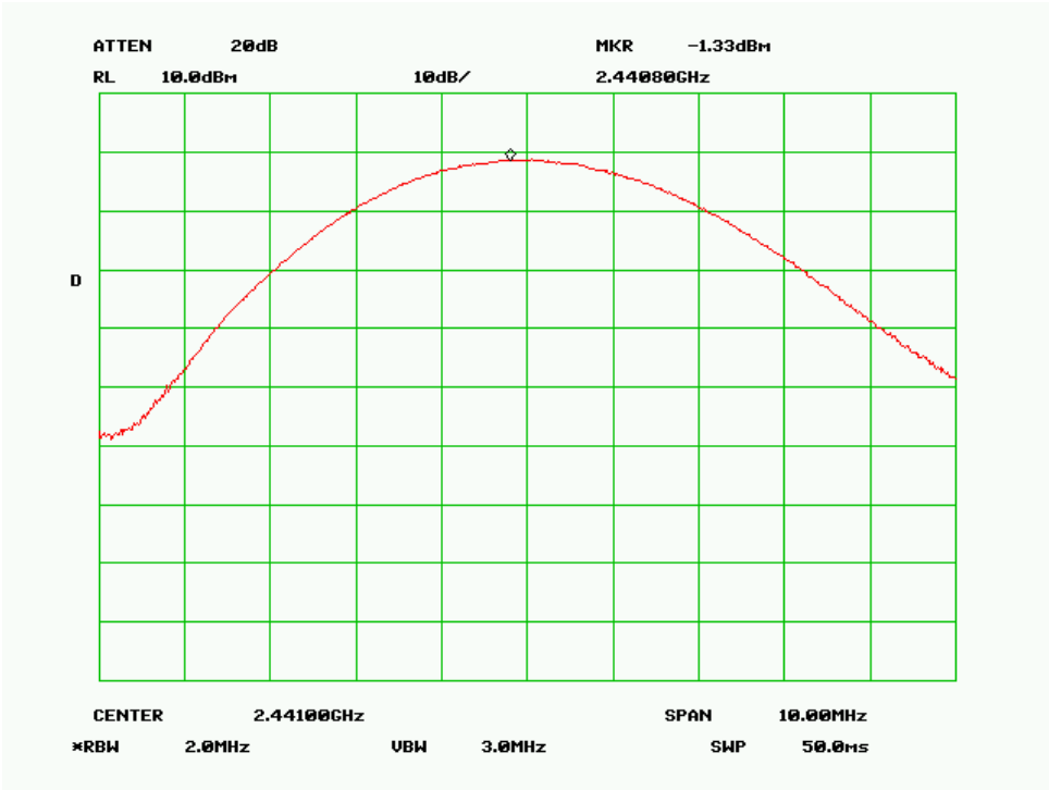
Output Power Mid Channel (Bluetooth)
