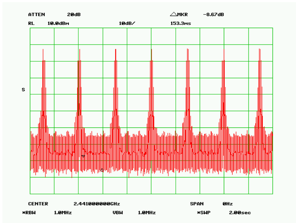
Middle Channel (Sweep in 2sec)
