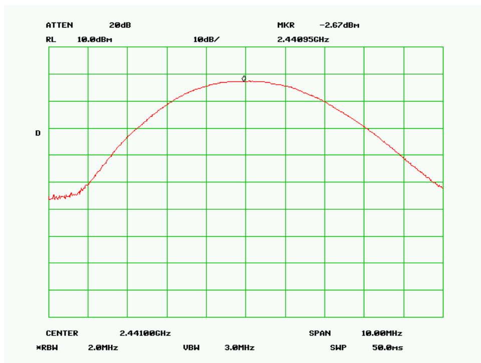
Output Power Middle Channel (Bluetooth)
