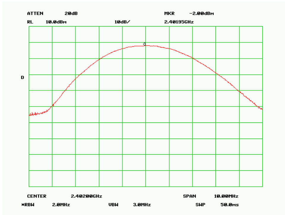
Output Power Low Channel (Bluetooth)
