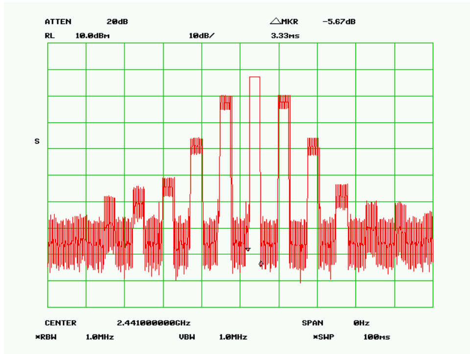
Middle Channel (Sweep in 100.0msec)
