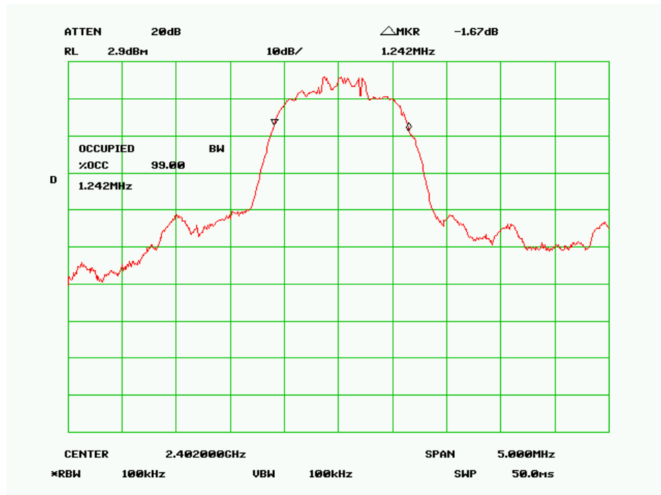
99% dB Bandwidth - Low Channel
