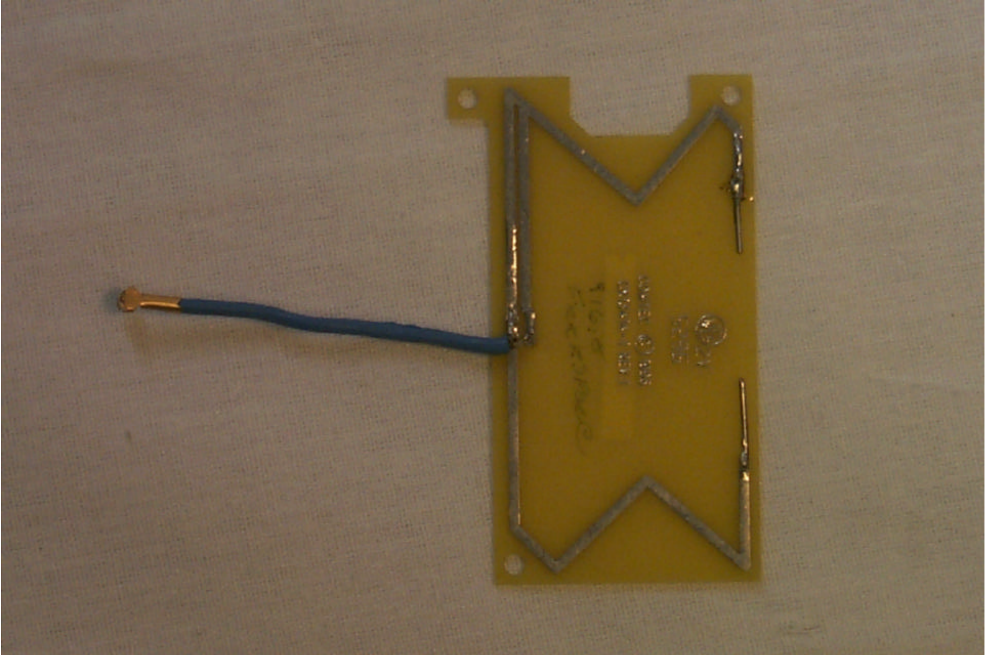
PCB Antenna
