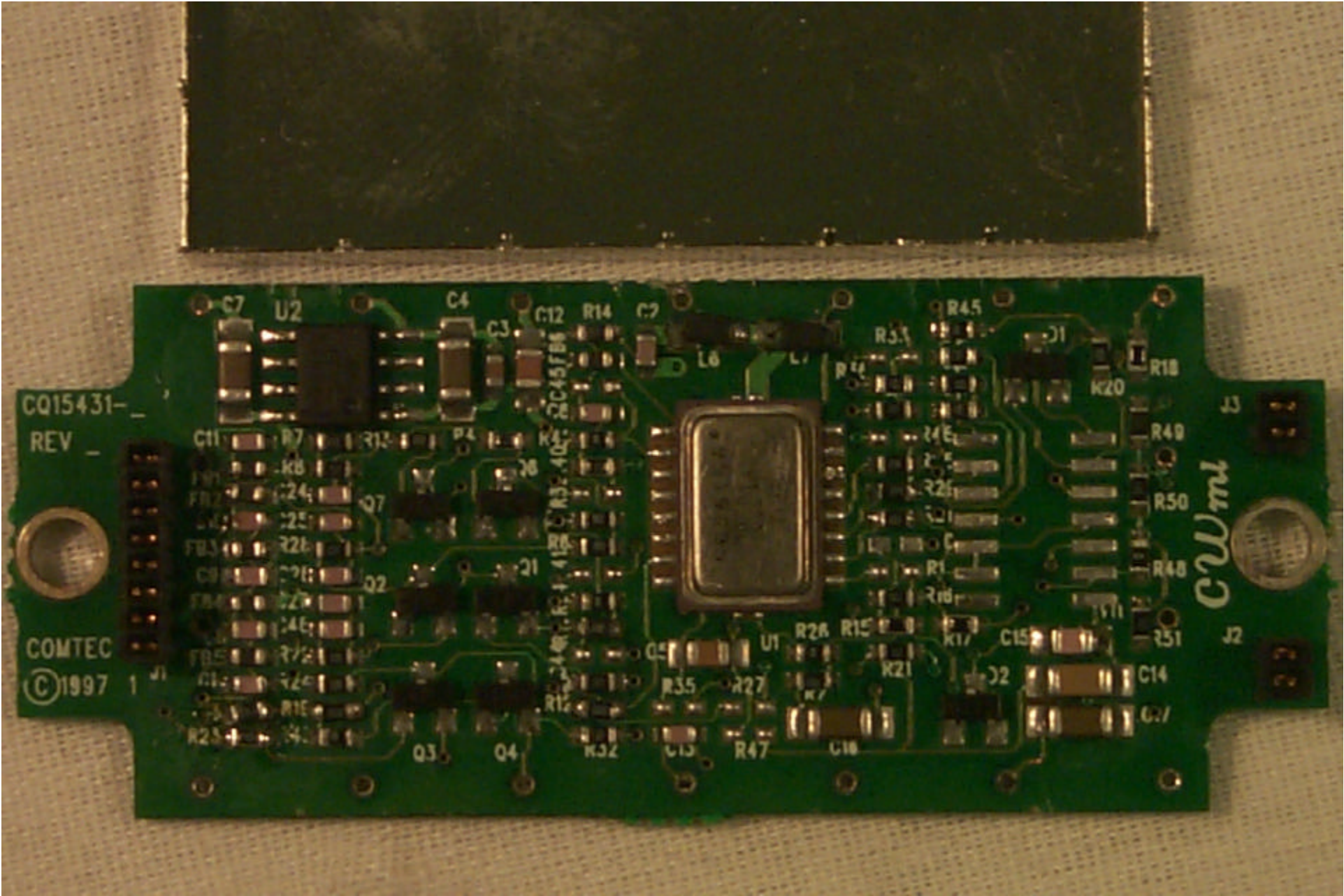
PCB Close-UP
