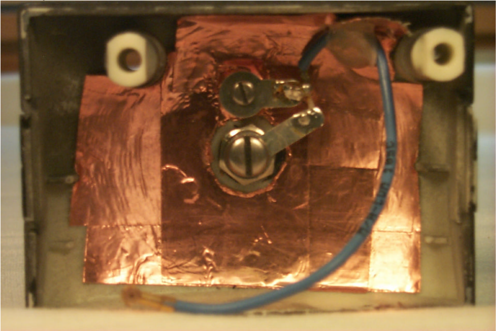
Inside of Monopole Antenna
