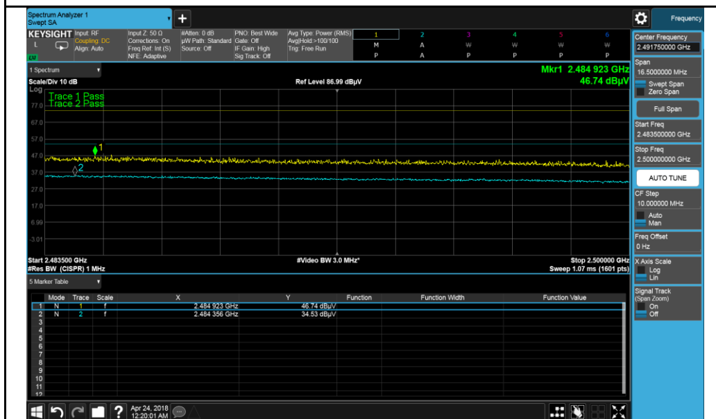
802.11n-HT40-2452MHz
