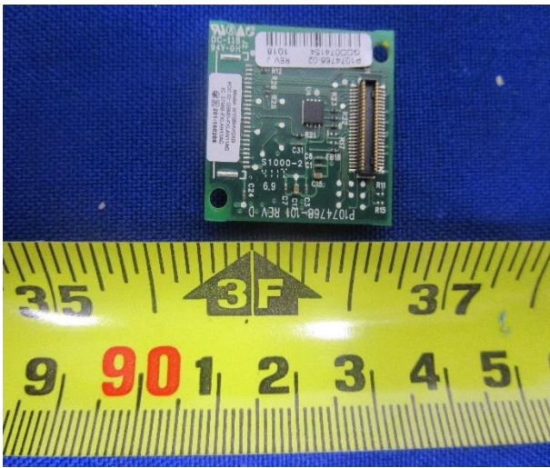
Radio Module - Top View
