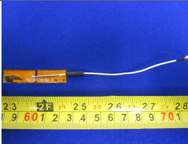
EUT AC Radio Version M/N: ZQ320 P/N: ZQ32-A0W01R0-001 Antenna - Top View
