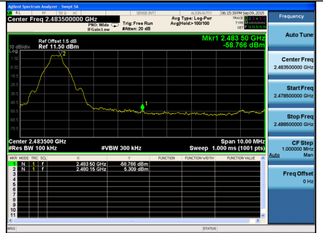
Band Edge-Single-BDR 2480MHz
