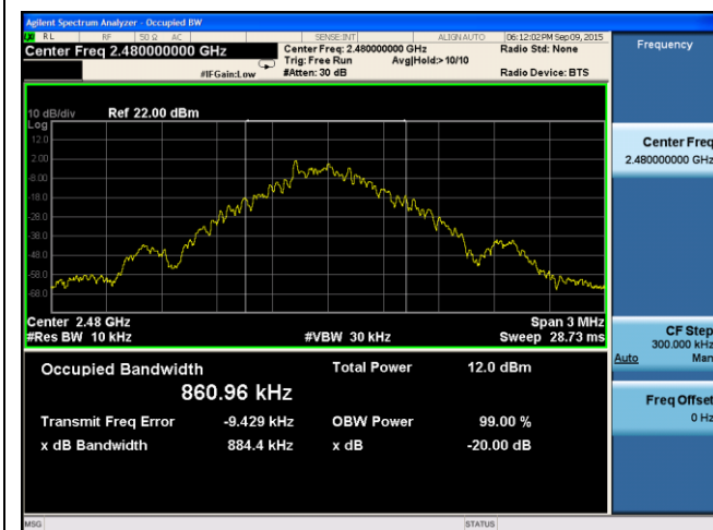
99% and 20dB BW –Bluetooth BDR 2480MHz
