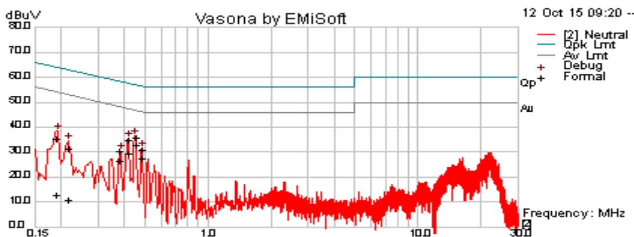
Neutral Plot at 120Vac, 60Hz
