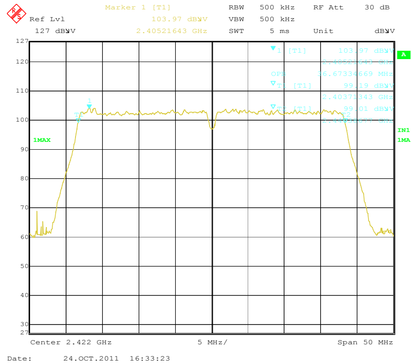
99% dB Bandwidth - 802.11n-40M-2.4G, Low Channel
