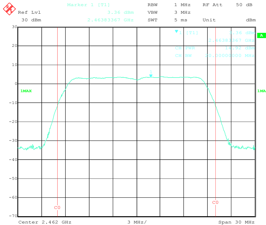
Output Power High Channel (802.11n-20MHz)
