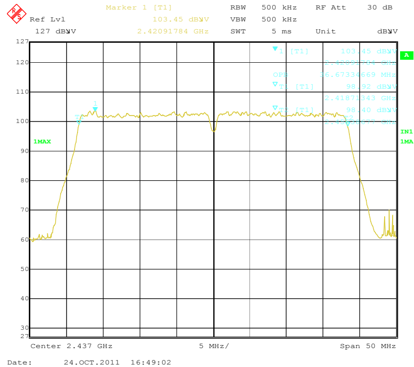
99% dB Bandwidth - 802.11n-40M-2.4G, Mid Channel
