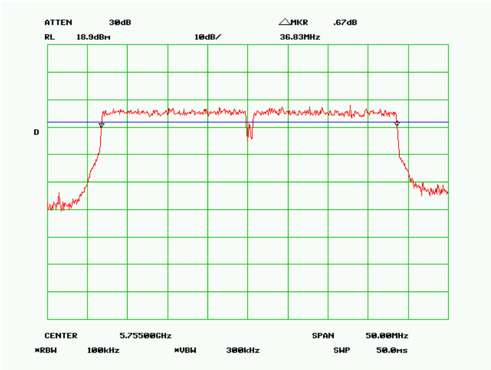
6 dB Bandwidth – 802.11n-40MHz 5.7G, Low Channel
