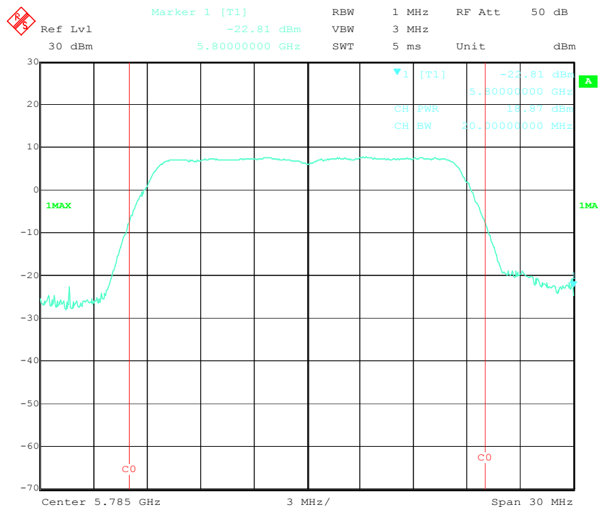
Output Power Mid Channel (802.11n-20MHz 5.7GHz)
