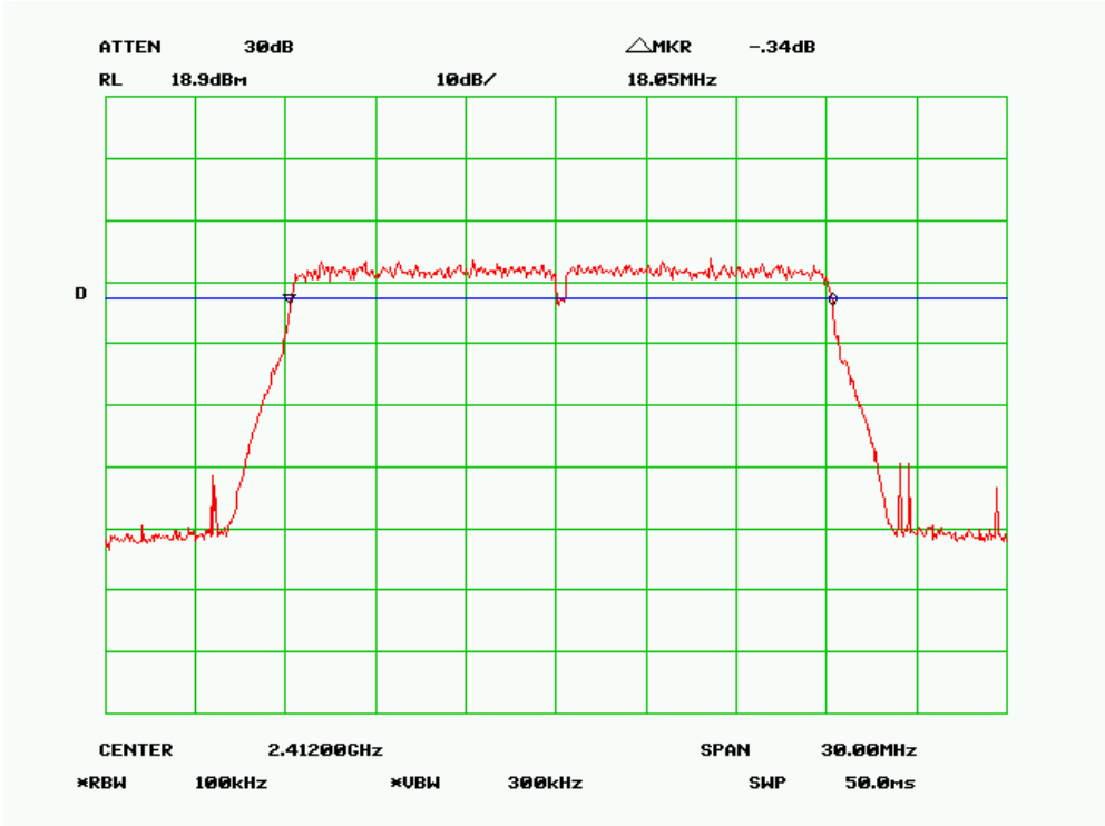
6 dB Bandwidth – 802.11n-20M-2.4G, Low Channel
