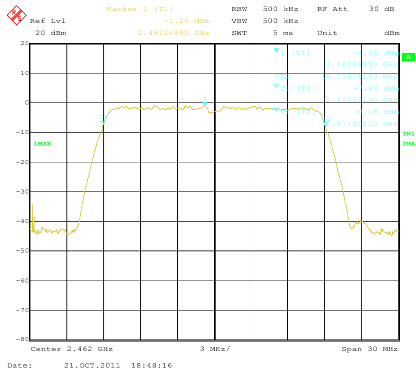
99% dB Bandwidth - 802.11n-20M-2.4G, High Channel
