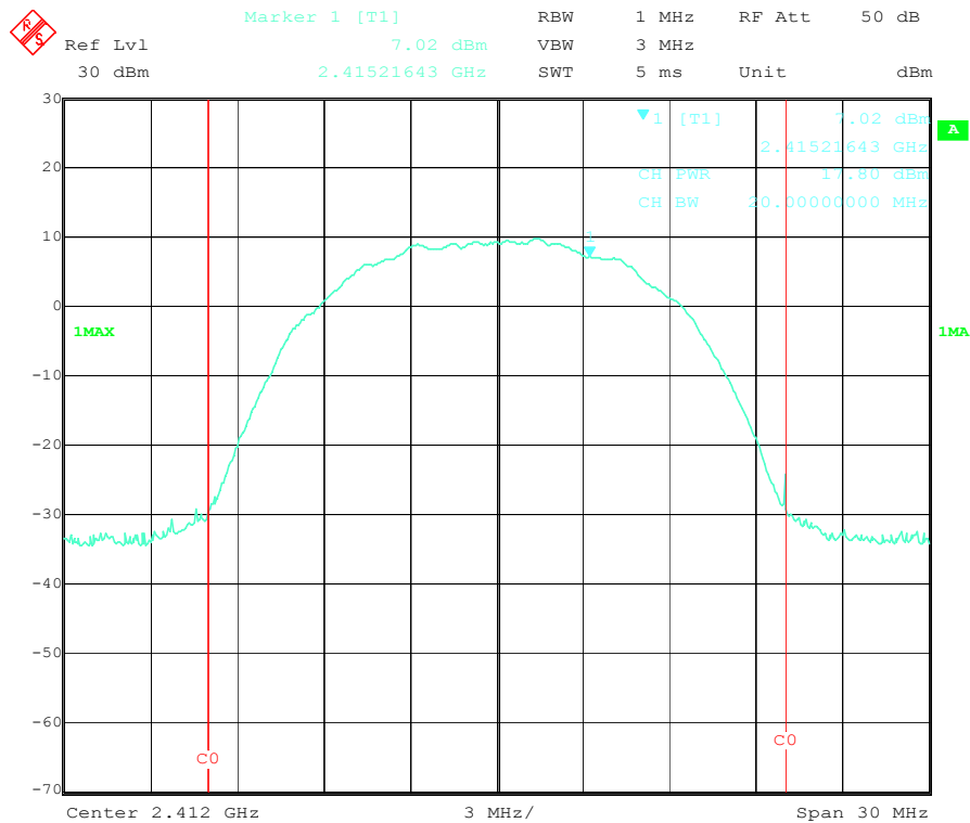
Output Power Low Channel (802.11b)
