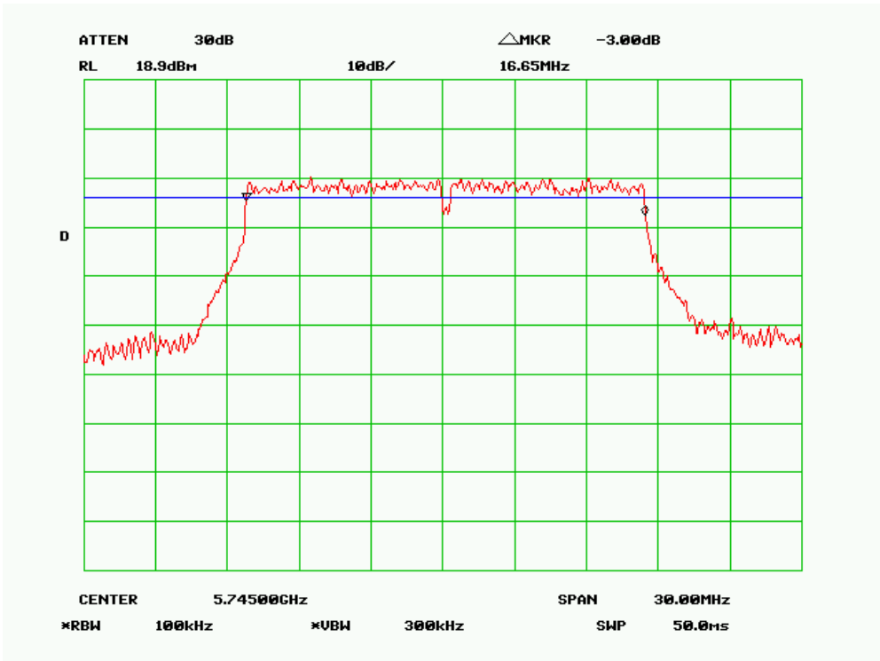
6 dB Bandwidth – 802.11a 5.7G, Low Channel
