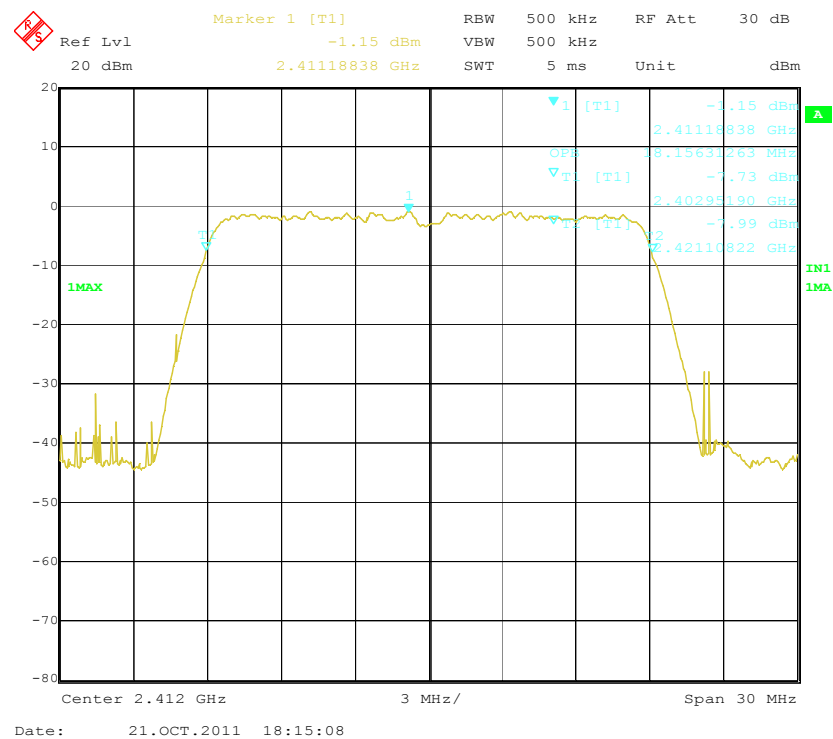
99% dB Bandwidth - 802.11n-20M-2.4G, Low Channel
