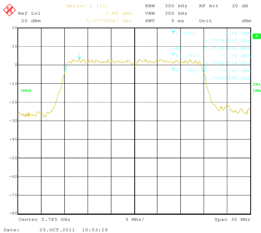
99% dB Bandwidth – 802.11a 5.7G, Mid Channel
