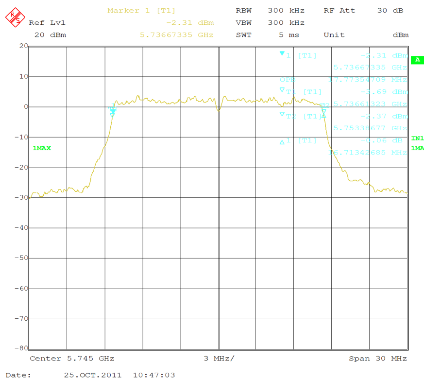
99% dB Bandwidth – 802.11n-20MHz 5.7G, Low Channel
