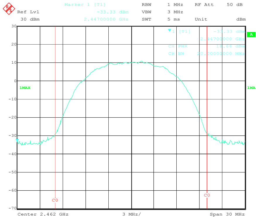
Output Power High Channel (802.11b)
