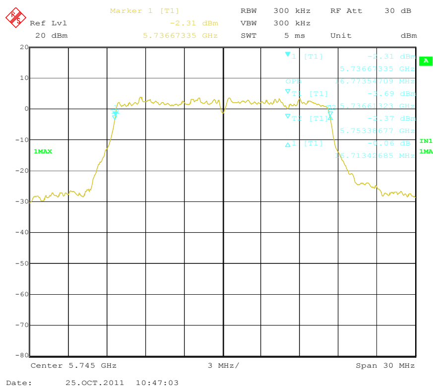
99% dB Bandwidth – 802.11a 5.7G, Low Channel
