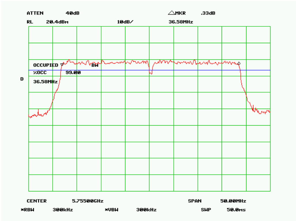
99% dB Bandwidth – 802.11n-40MHz 5.7G, Low Channel
