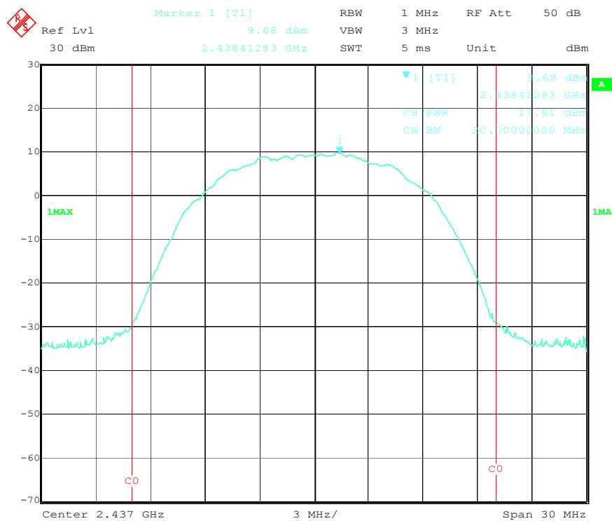
Output Power Middle Channel (802.11b)
