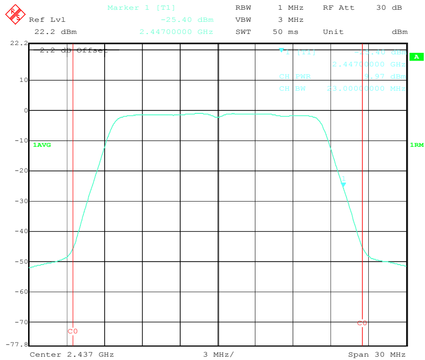
Output Power Middle Channel (802.11g)
