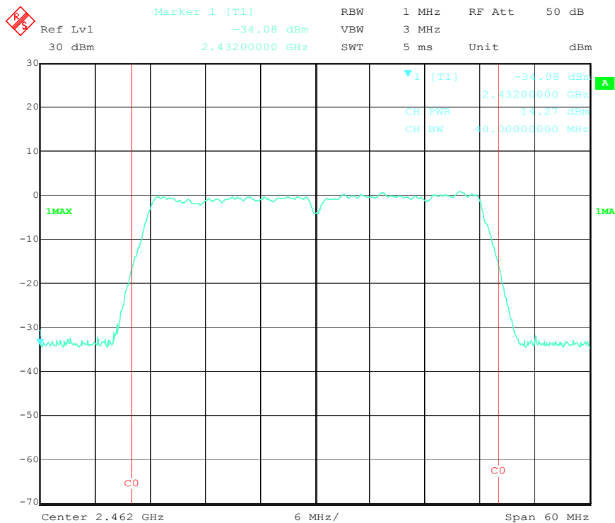
Output Power High Channel (802.11n-40MHz)
