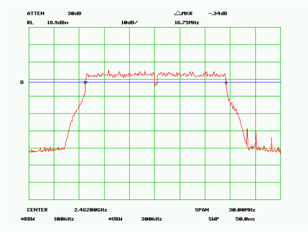
6 dB Bandwidth – 802.11g, High Channel
