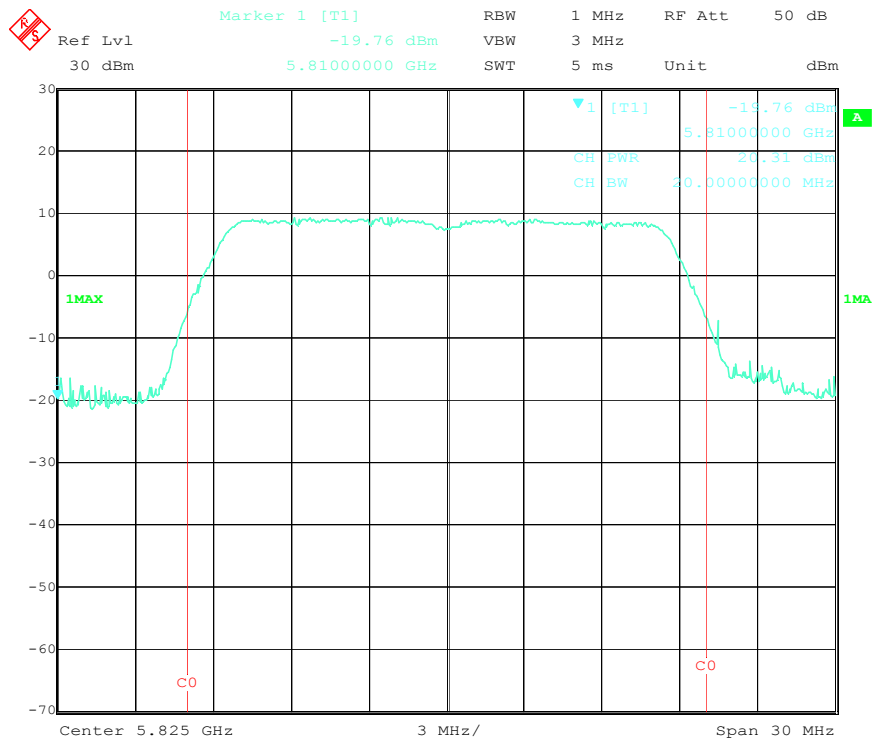
Output Power High Channel (802.11n-20MHz 5.7GHz)
