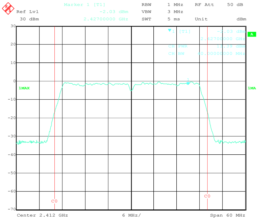
Output Power Low Channel (802.11n-40MHz)
