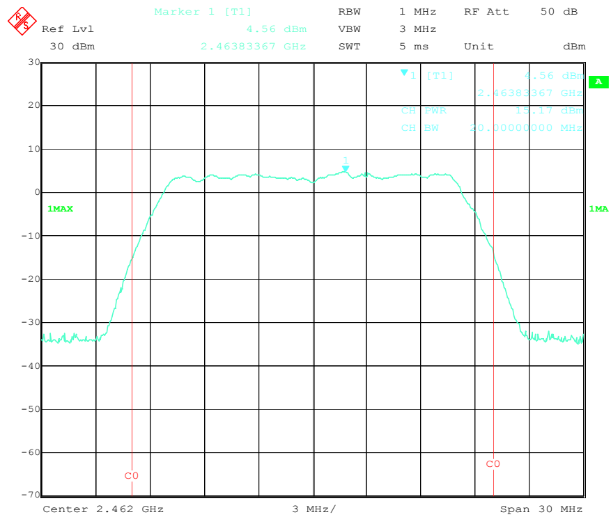
Output Power High Channel (802.11g)
