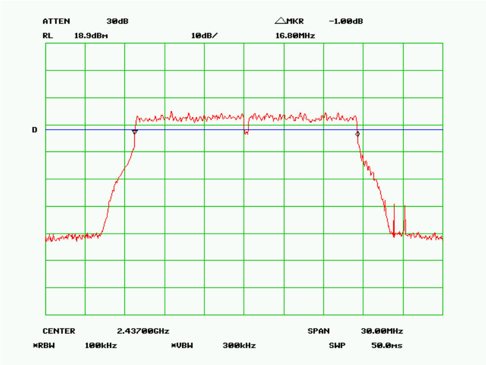
6 dB Bandwidth - 802.11g, Middle Channel
