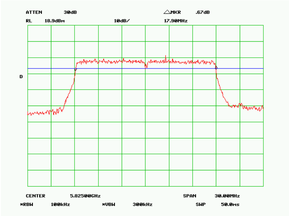
6 dB Bandwidth – 802.11n-20MHz 5.7G, High Channel
