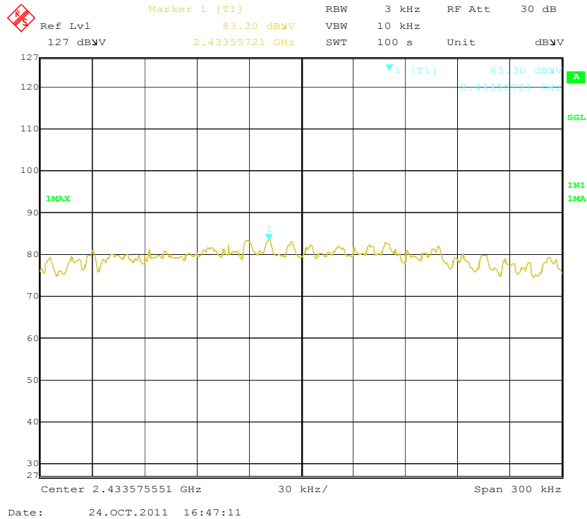
PSD Mid Channel (802.11n-40MHz-2.4G)
