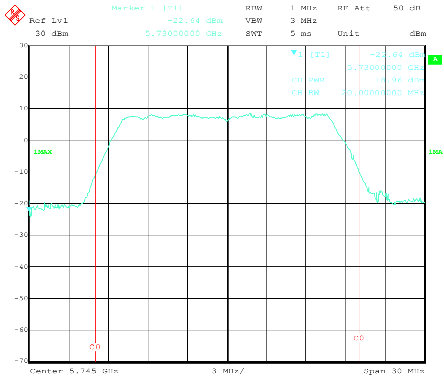
Output Power Low Channel (802.11a)
