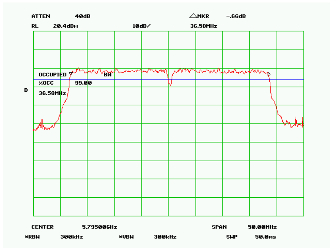
99% dB Bandwidth – 802.11n-40MHz 5.7G, High Channel
