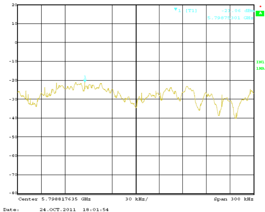
PSD High Channel (802.11n-40MHz 5.7GHz)
