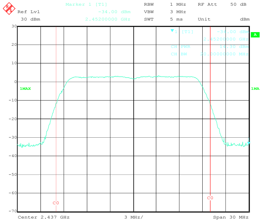
Output Power Middle Channel (802.11n-20MHz)
