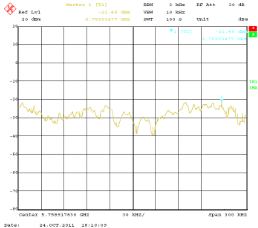
PSD Low Channel ( 802.11n-40MHz 5.7GHz)
