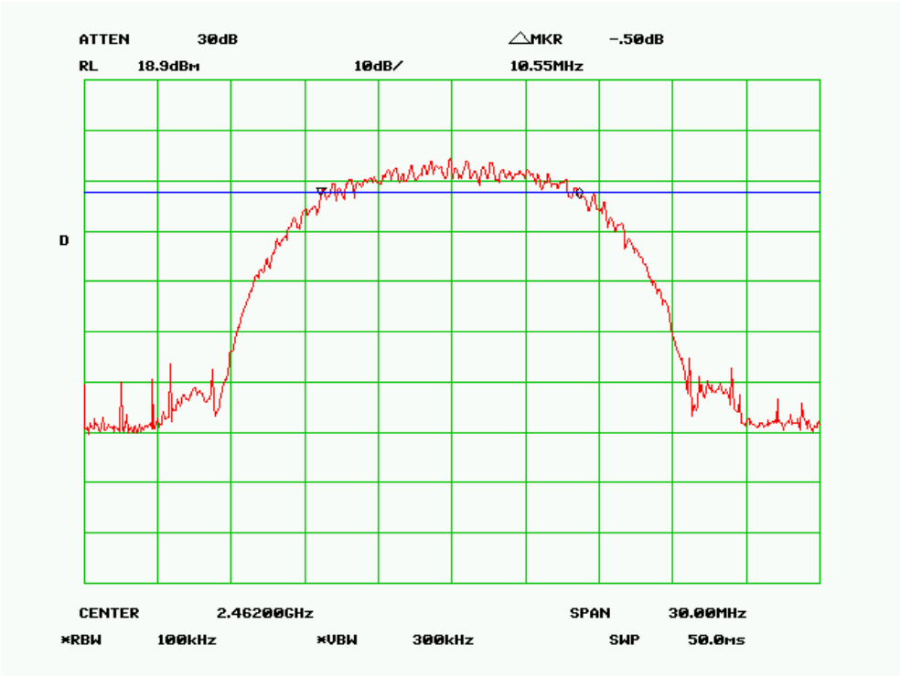
6 dB Bandwidth – 802.11b, High Channel
