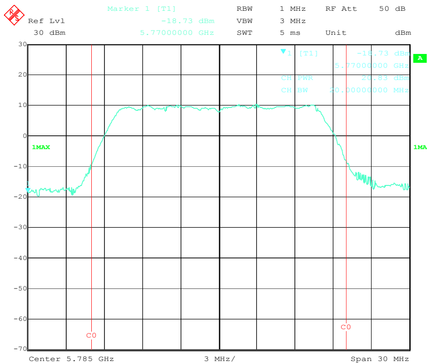
Output Power Middle Channel (802.11a)
