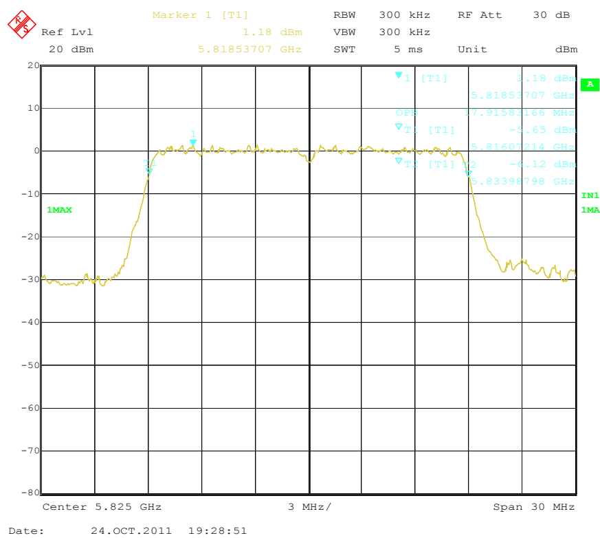
99% dB Bandwidth – 802.11n-20MHz 5.7G, High Channel
