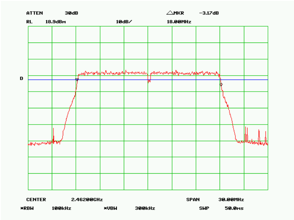
6 dB Bandwidth – 802.11n-20M-2.4G, High Channel
