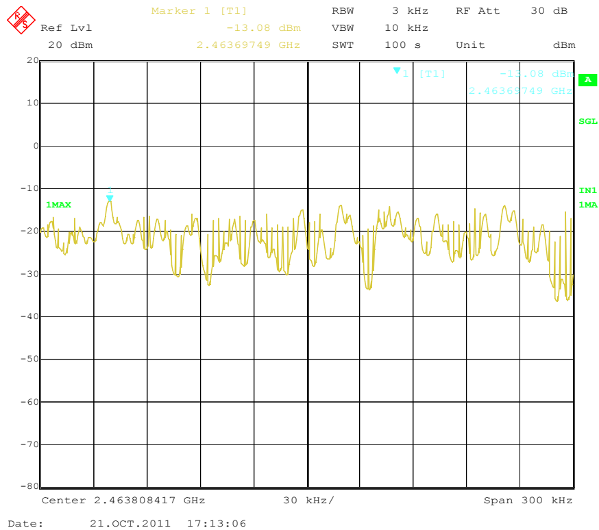
PSD High Channel ( 802.11b)
