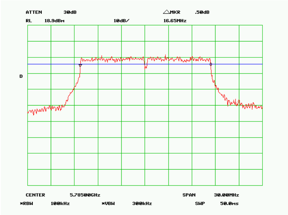
6 dB Bandwidth – 802.11a 5.7G, Mid Channel
