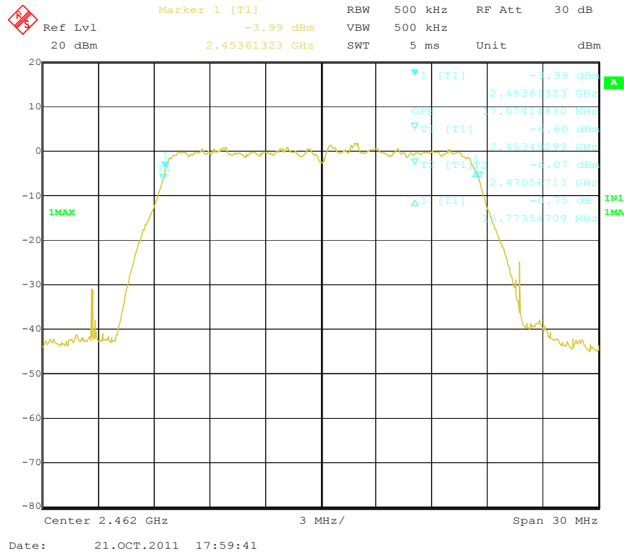
99% dB Bandwidth - 802.11g, High Channel
