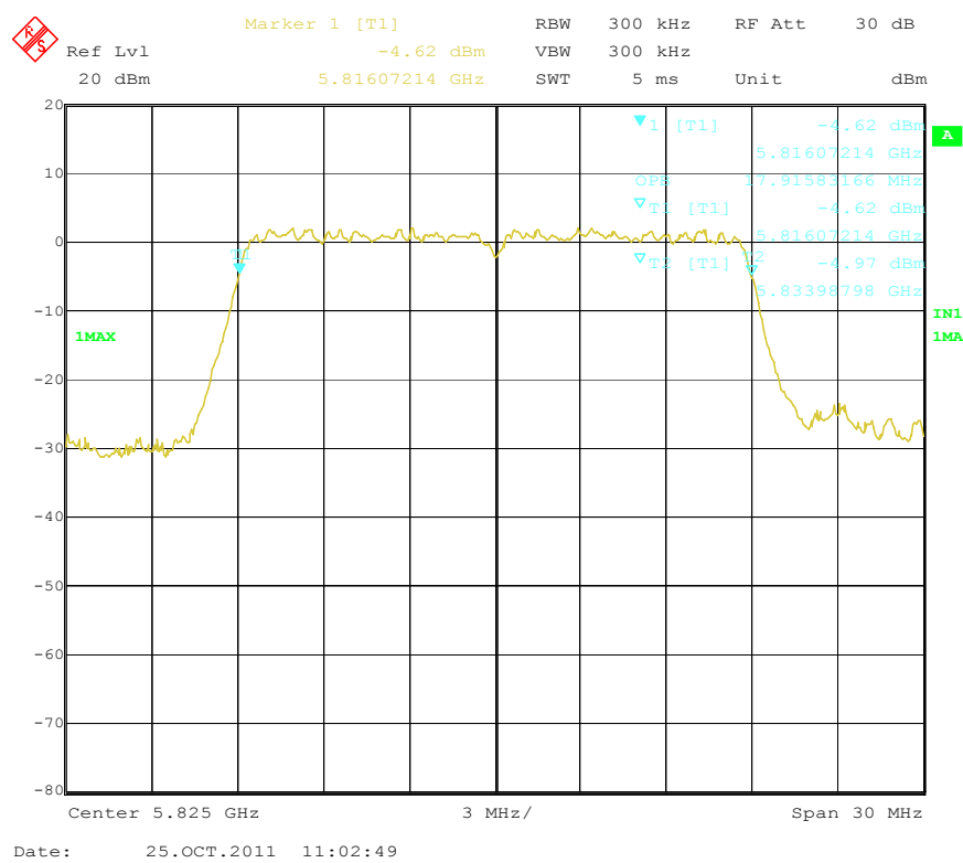
99% dB Bandwidth – 802.11a 5.7G, High Channel
