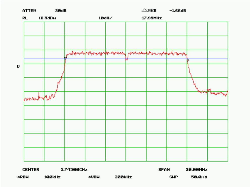
6 dB Bandwidth – 802.11n-20MHz 5.7G, Low Channel
