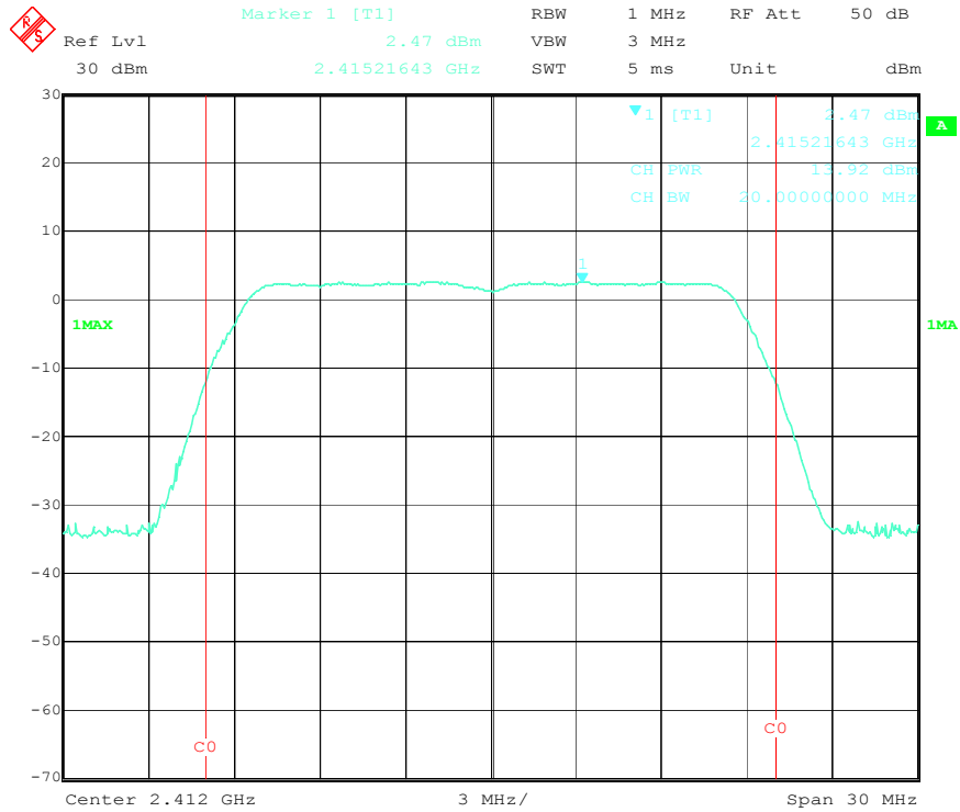
Output Power Low Channel (802.11n-20MHz)
