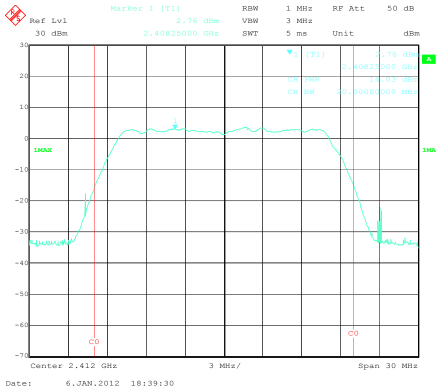
Output Power Low Channel (802.11g)
