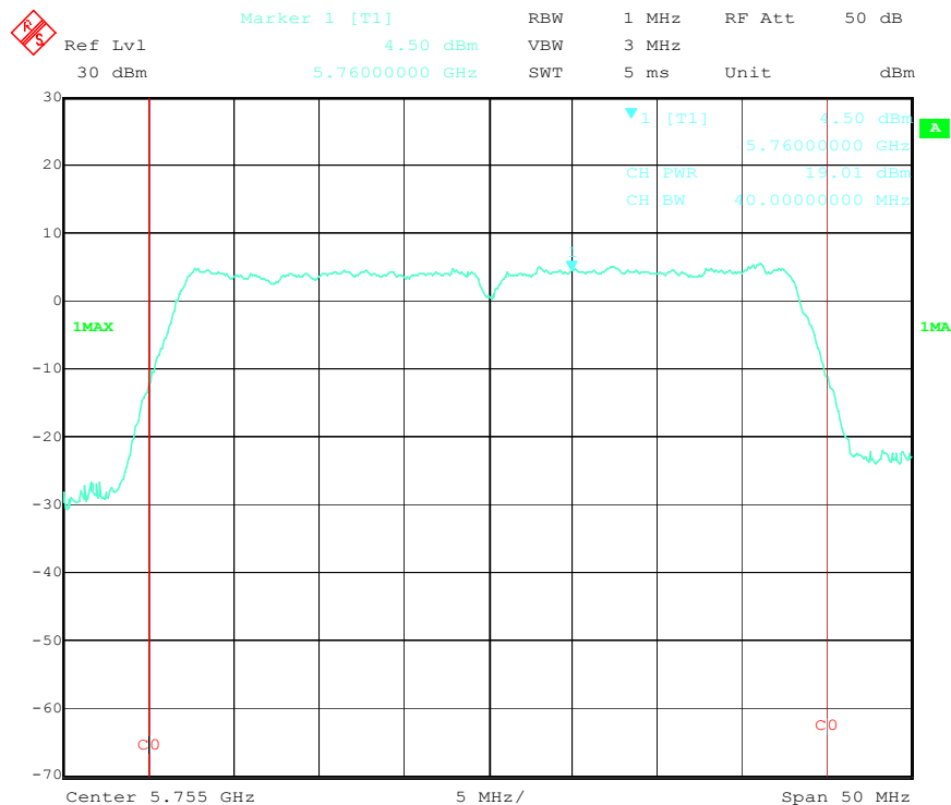
Output Power Low Channel ( 802.11n-40MHz 5.7GHz)
