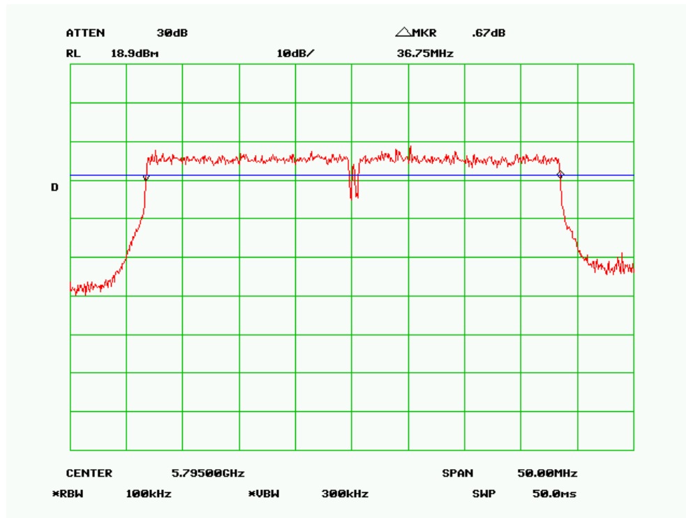
6 dB Bandwidth – 802.11n-40MHz 5.7G, High Channel
