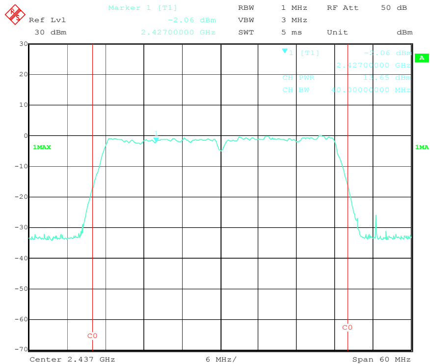
Output Power Mid Channel (802.11n-40MHz)
