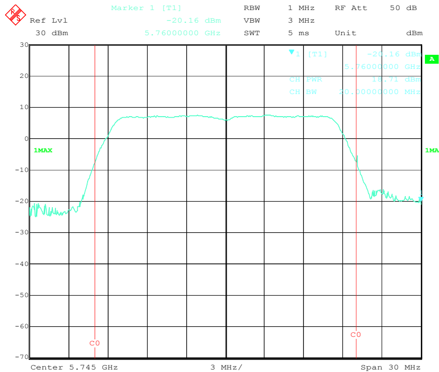
Output Power Low Channel ( 802.11n-20MHz 5.7GHz)
