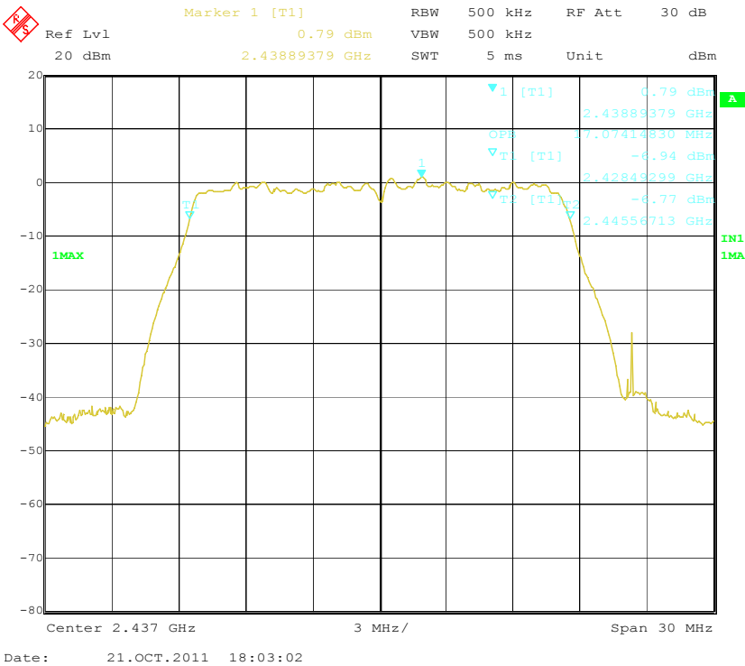
99% dB Bandwidth - 802.11g, Mid Channel
