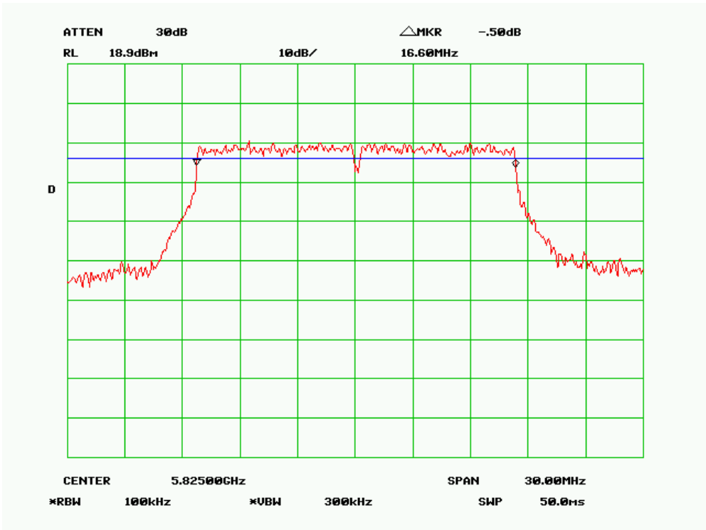
6 dB Bandwidth – 802.11a 5.7G, High Channel
