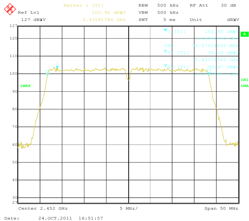
99% dB Bandwidth - 802.11n-40M-2.4G, High Channel
