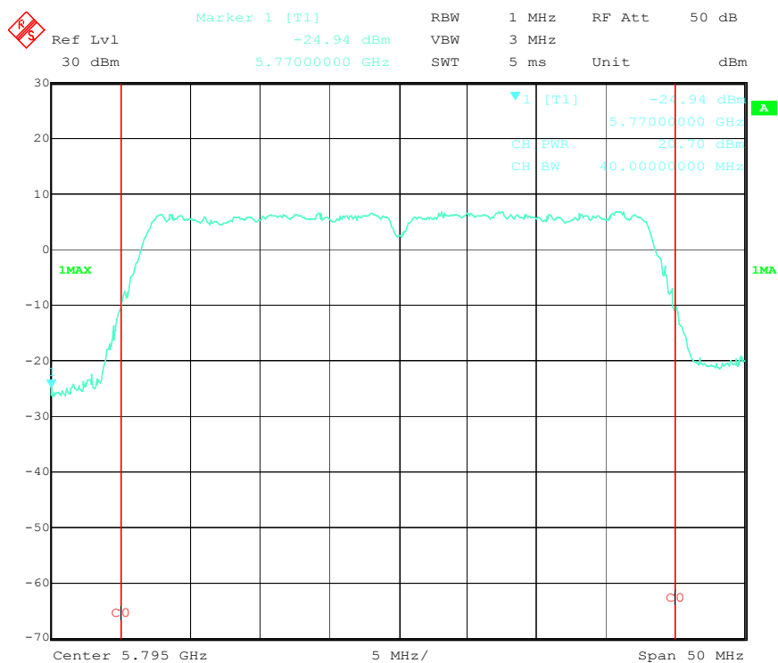
Output Power High Channel (802.11n-40MHz 5.7GHz)
