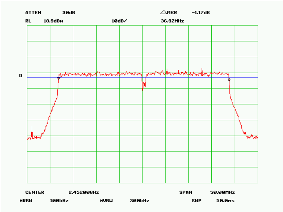
6 dB Bandwidth – 802.11n-40M-2.4G, High Channel
