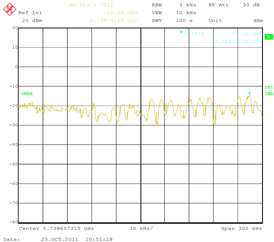
PSD Low Channel ( 802.11a 5.7GHz)
