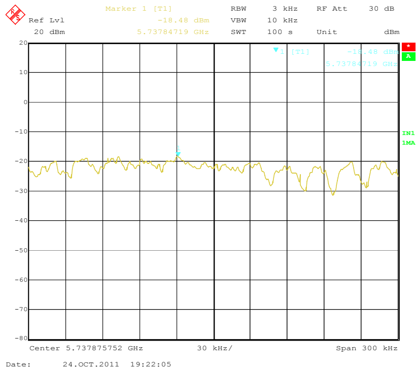
PSD Low Channel ( 802.11n-20MHz 5.7GHz)
