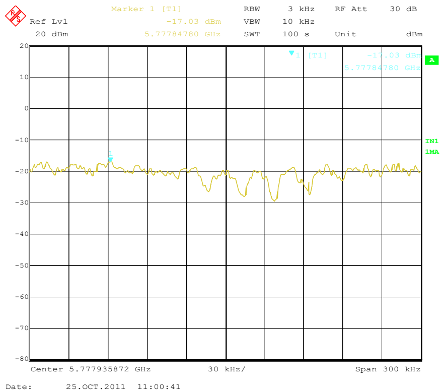
PSD Mid Channel (802.11a 5.7GHz)
